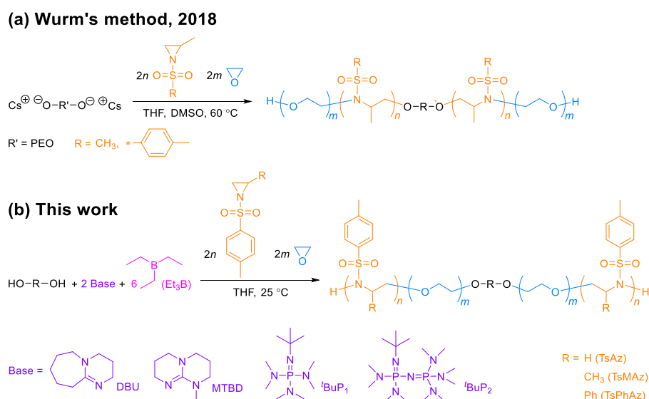
Scheme 1. General scheme for one-step block copolymerization of EO and Az by (a) cesium alkoxide-initiated anionic copolymerization following an Az-first order and (b) alcohol-initiated metal-free copolymerization following a reverse (EO-first) order.
