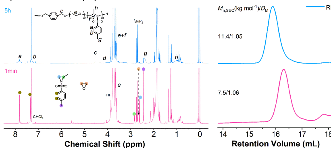
Figure 1. 1 H NMR spectra (left) and SEC traces (right) of the aliquots withdrawn at different reaction times for entry 2 in Table 1.
