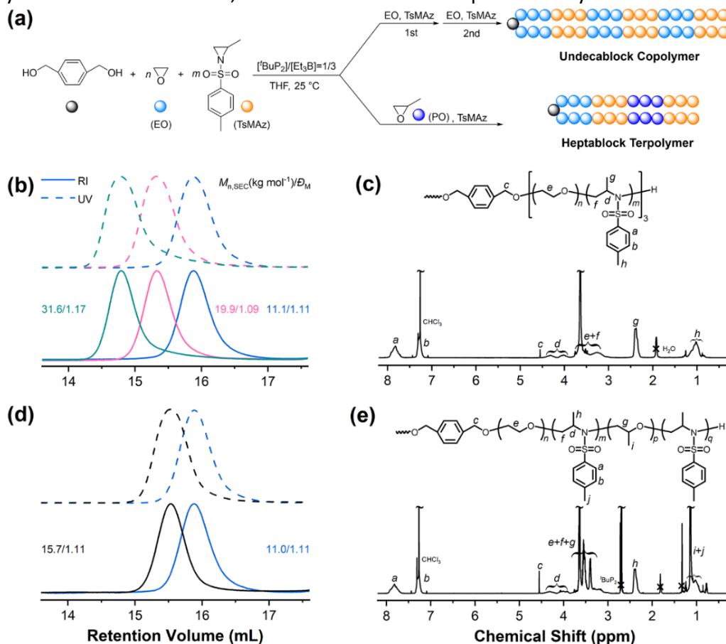
Figure 2. (a) One-pot multiblock co-/terpolymer synthesis (entry 10 and 11 in Table 1); (b) SEC traces after full consumption of each batch of EO/TsMAz; (c) ^1\text{H} NMR spectrum of the undecablock copolymer; (d) SEC traces after full consumption of EO/TsMAz and PO/TsMAz; (e) ^1\text{H} NMR spectrum of the heptablock terpolymer
