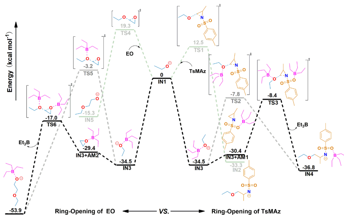
Figure 3. Modelling of the reaction between an oxyanion and EO (left) or TsMAz (right) in the presence of different amounts of Et 3 B. Light grey line: [Et 3 B] = 0; dark grey line: [Et 3 B]/[oxyanion] = 1, black line: [Et 3 B]/[oxyanion] = 3.
