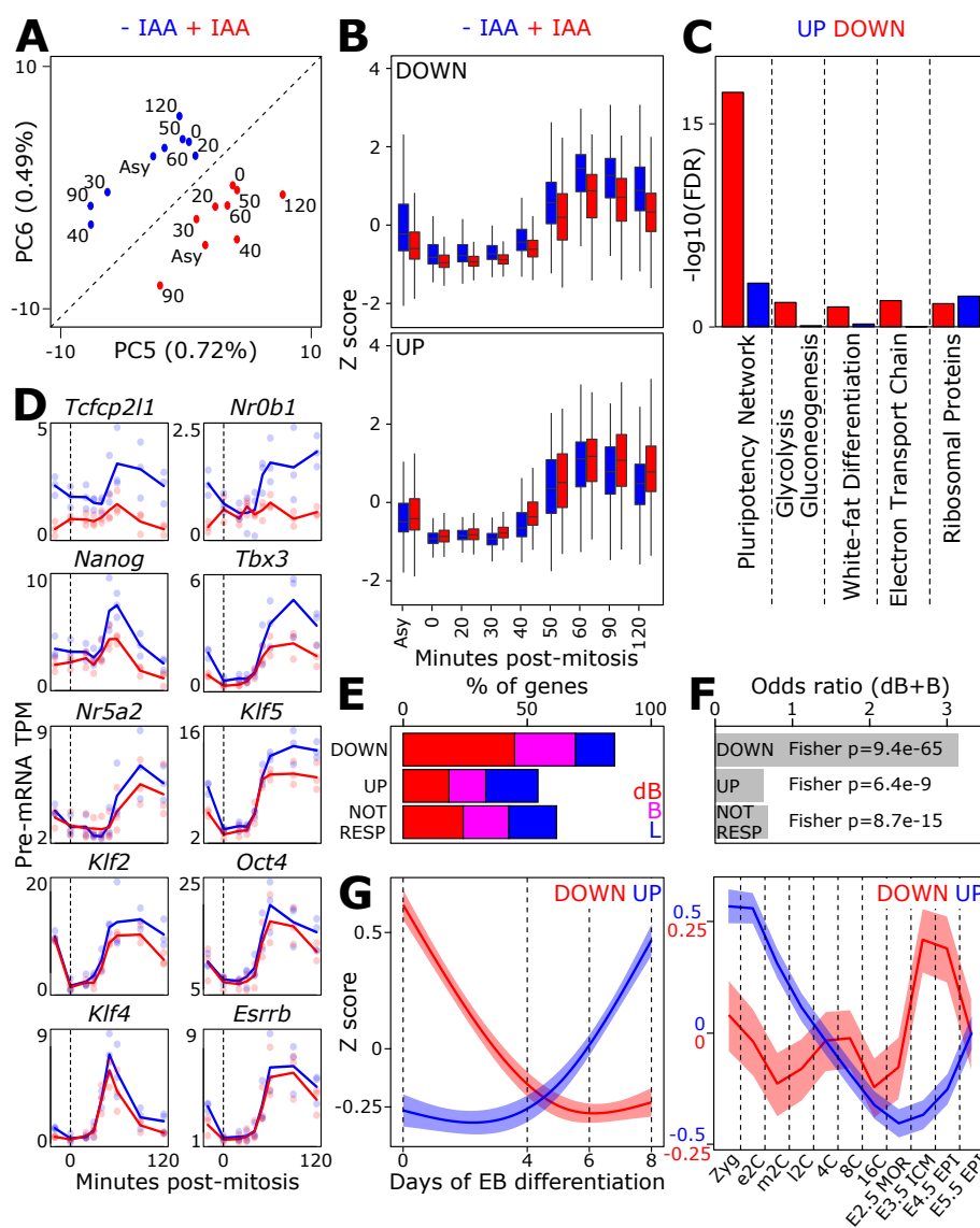
Fig. 6. Mitotic bookmarking by ESRRB/NR5A2 promotes the reactivation of genes associated with pluripotency. (A) PCA analysis of post-mitotic gene transcription dynamics of cells exiting mitosis in either the presence (-IAA) or absence (+IAA) of ESRRB/NR5A2. PC5 and PC6 capture ESRRB/NR5A2-dependent differences. (B) Post-mitotic gene transcription dynamics of genes derived from the loadings of PC5/PC6 and displaying either a downregulation or an upregulation upon ESRRB/NR5A2 depletion. (C) Gene ontology analyses of the gene groups shown in (B). (D) Examples of post-mitotic gene reactivation dynamics for genes belonging to the pluripotency network, in the presence (blue) or the absence (red) of ESRRB/NR5A2. (E) Percentage of genes associated with ESRRB/NR5A2 dB, B (eB+nB) or L regions, for extended sets identified as downregulated, upregulated or not responsive. (F) Statistical analysis of the association of the sets shown in (E) with bookmarked regions (dB+eB+nB). (G) Mean expression profile during Embryoid Body differentiation (left) or Early Mouse Embryogenesis (right) of genes downregulated or upregulated upon ESRRB/NR5A2 depletion during the M-G1 transition (Zyg: Zygote; e/m/12C: early/mid/late 2 cell stage; 4/8/16C: 4/8/16 cell stage; MOR: Morula; ICM: Inner Cell Mass; EPI: Epiblast).
