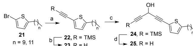
Scheme 6. Synthesis of 2,5-thienyl PAC analogues 25 via route A a
