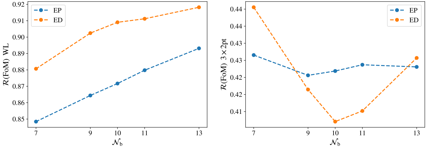
Fig. 10. FoM ratio vs the number of EP and ED redshift bins for WL (left) and 3 \times 2\text{pt} (right) in the optimistic scenario. The blue curves in this plot match the ones in the bottom right panel of Fig 9 in the optimistic case, for the corresponding probes.
