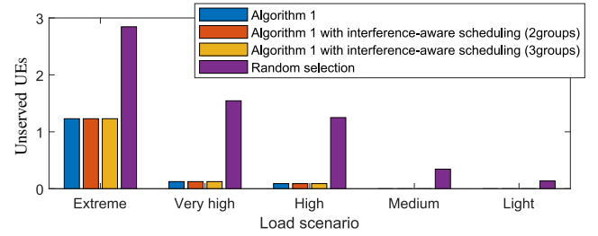
b) Average number of unserved UEs vs different cases of buffer overflow.
