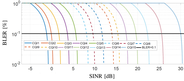
Fig. 2: BLER - CQI mapping defined as “Table-1”.
