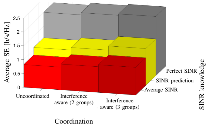
Fig. 6: Improvement in average SE by incorporating smart LA and interference aware scheduling.
