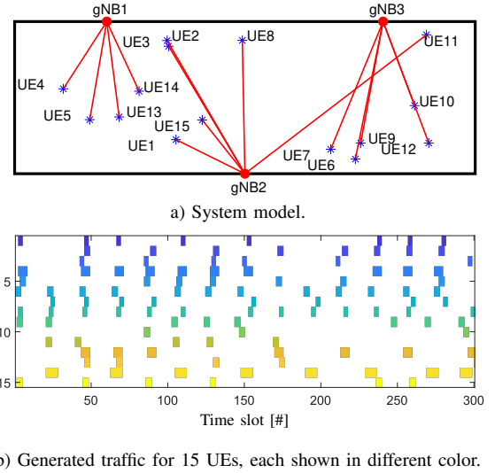
Fig. 1: Traffic model.
