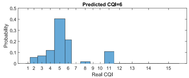
Fig. 3: Actual CQI when LSTM prediction corresponds to CQI=6, i.e., \Pr(\text{CQI}_r = y|x = 6) for y = 0, \dots, 15 .
