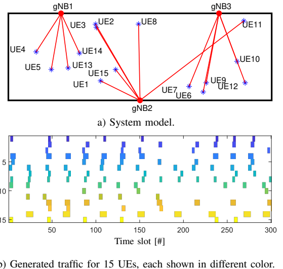
Fig. 1: Traffic model.
