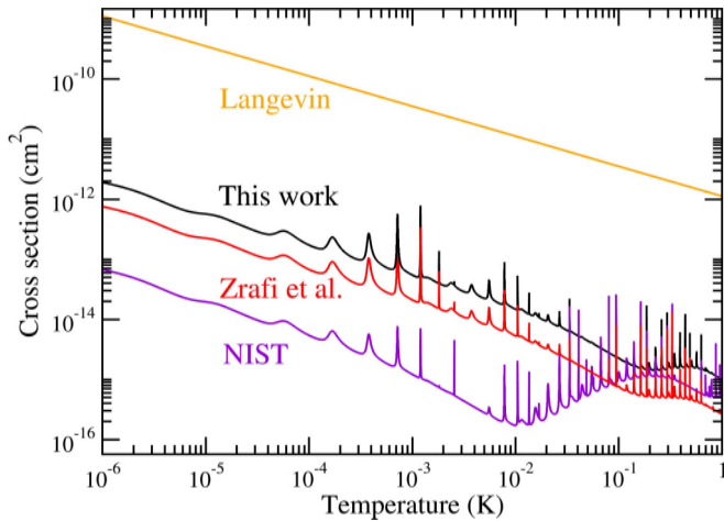
FIG. 12. NRCE cross sections obtained after the shift of the energy D_f of the dissociation limit of the exit channel 1^3\Pi PEC to D_f(\text{NIST}) (violet) and to D_f ([29]) (red) compared to the present value (black). The Langevin cross section \sigma_L (orange) is plotted for comparison.
