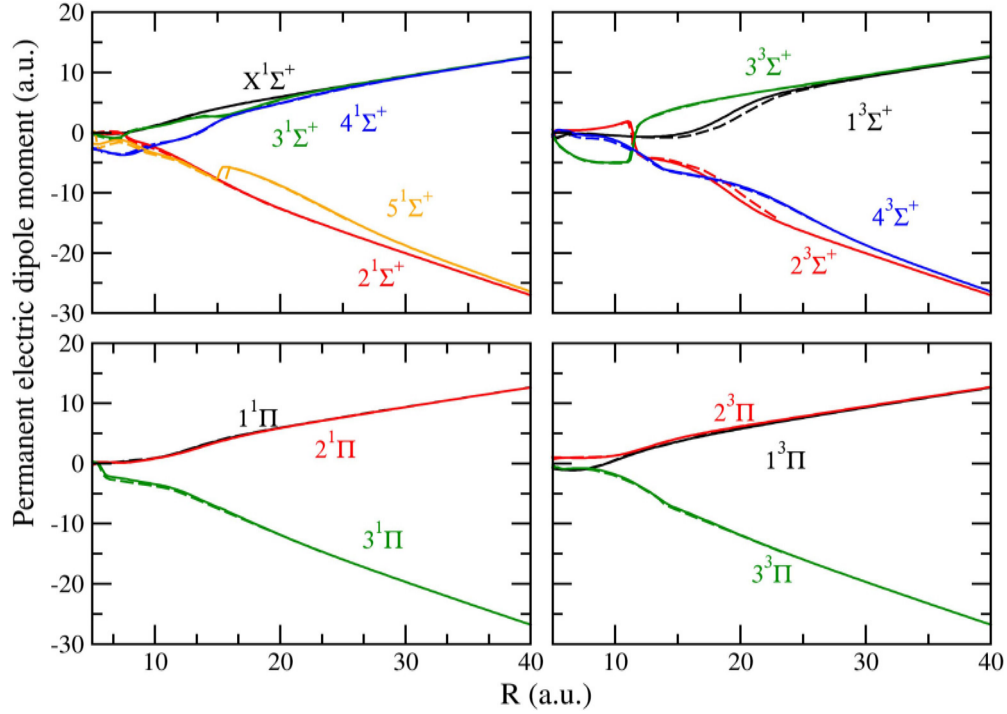
FIG. 13. Selected PEDMs computed in this paper (solid lines) compared to Ref. [29] (dashed lines).
