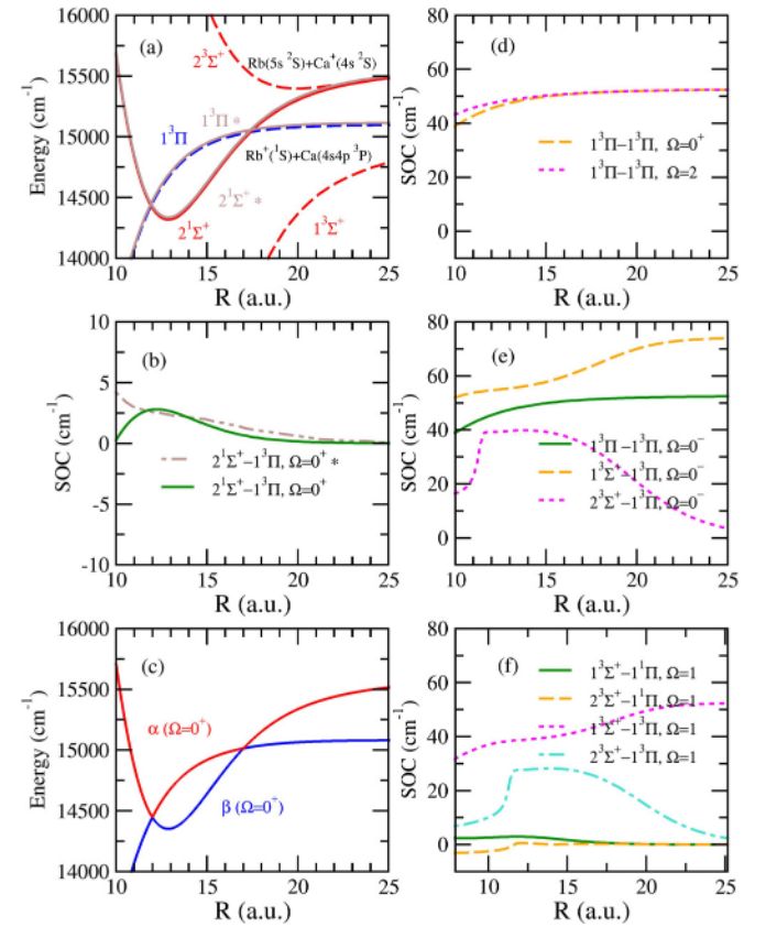
FIG. 4. (a) Magnified view of the \text{RbCa}^+ PECs involved in the NRCE process \text{Rb}(5s^2S) + \text{Ca}^+(4s^2S) \rightarrow \text{Rb}^+ + \text{Ca}(4s4p^3P) . The theoretical results from Ref. [27] are labeled by a star * (brown line). (b) SOC between the 2^1\Sigma^+ and the 1^3\Pi states computed in the present work for the \Omega = 0^+ symmetry, together with the one computed in Ref. [27] (labeled with a star *, dashed brown line). (c) Adiabatic PECs resulting from the diagonalization of the \mathbf{H}_{\text{eff}}(\Omega^p; R) matrix (see the main text). (d) Diagonal SOC for the \Omega = 0^+, 2 symmetries. (e) SOC for the \Omega = 0^- symmetry. (f) SOC for \Omega = 1 symmetry. Note that the kinks in the coupling between 2^3\Sigma^+ and 1^3\Pi visible in (e) and (f) are due to the avoided crossing around 12 a.u. of the 2^3\Sigma^+ and 3^3\Sigma^+ PECs (see Fig. 2.)
