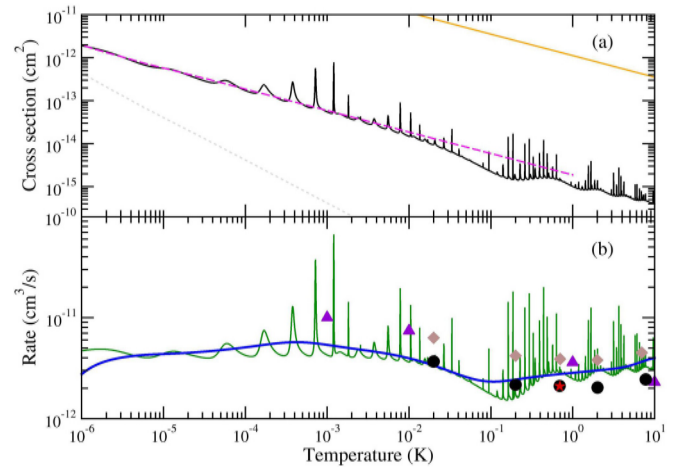
FIG. 10. (a) Computed cross section (solid black curve) for the NRCE process \text{Rb}(5s^2S) + \text{Ca}^+(4s^2S) \rightarrow \text{Rb}^+(^1S) + \text{Ca}(4s4p^3P) as a function of the temperature T = E_{\text{coll}}/k_B related to the relative collision energy E_{\text{coll}} compared to the Langevin cross section (solid orange line) and to the expression of Eq. (9) (first term: dotted grey line; second term: dashed magenta line). (b) Nonthermalized (solid green oscillatory line) and Boltzmann-thermalized (superimposed solid blue line) NRCE rate coefficients compared to the theoretical results of Ref. [27] averaged with a Boltzmann distribution (violet triangles), with the distribution determined by the ion velocities (brown diamonds, see Fig. 5(c) of Ref. [5]), to the down-scaled experimental data (black circles) of Ref. [4] (see text), and to the experimental value at 2 K of Ref. [4] (red star).
