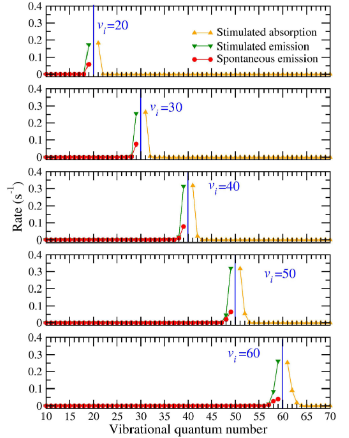
FIG. 7. Rates for spontaneous (stimulated) emission and absorption for the X 1 Σ + ground state vibrational levels v_i = 20, 30, 40, 50, 60 toward every X 1 Σ + final level v_f for J_i = 0 \rightarrow J_f = 1 .
