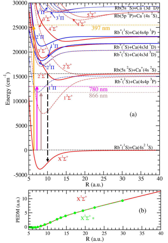
FIG. 2. (a) Hund's case a \text{RbCa}^+ PECs as functions of internuclear distance R . The origin of energies is taken at the asymptote of the electronic ground state \text{Rb}^+(^1S) + \text{Ca}(4s^2^1S) . The length of the vertical solid upward arrows represent the energies of the lasers present in the experiment [2] with wavelengths 397 nm (orange arrow), 780 nm (magenta arrow), and 866 nm (brown arrow). The black dashed downward arrow holds for the radiative association process (see the main text), resulting in the formation of \text{RbCa}^+ ions. (b) PEDM of the X^1\Sigma^+ state (solid red line) computed with the origin of distance taken at the \text{RbCa}^+ center of mass compared to the theoretical results of Ref. [29] (closed green dots).
