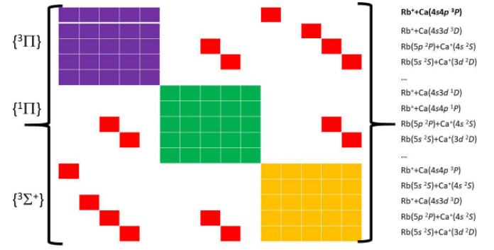
FIG. 3. A schematic representation of the effective Hamiltonian matrix \mathbf{H}_{\text{eff}} , illustrated for the case of \Omega = 1 . Three diagonal blocks (in purple, green, and orange) are present for the three relevant Hund's case a symmetries ^3\Pi, ^1\Pi , and ^3\Sigma^+ , respectively, while the atomic SOC (red squares) are connecting states from different blocks correlated with the same dissociation limit (thus the same fine-structure manifold).
