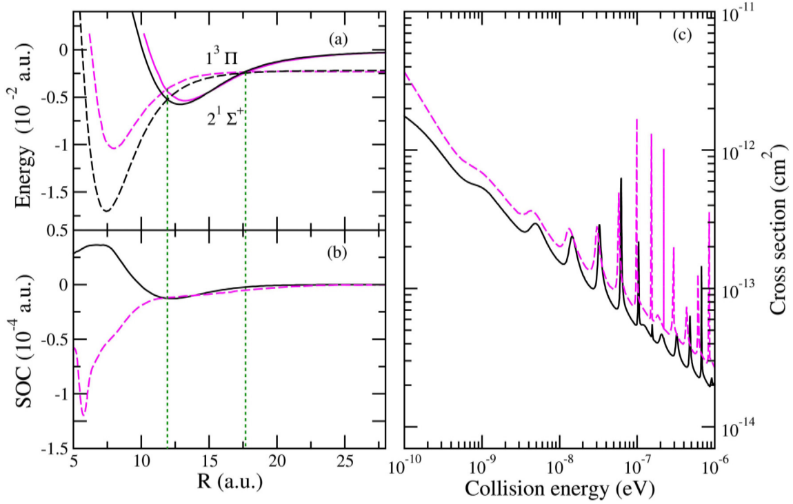
FIG. 15. This work (black) and Ref. [28] (magenta): (a) Hund's case a PECs of the 1^3\Pi (dashed line) and 2^1\Sigma^+ (solid line) states, the vertical dashed lines indicate the two crossings; (b) SOC between the 1^3\Pi and 2^1\Sigma^+ states, the vertical dashed lines mark the values of SOC at the two crossings; (c) The calculated NRCE cross sections as a function of the collision energy.
