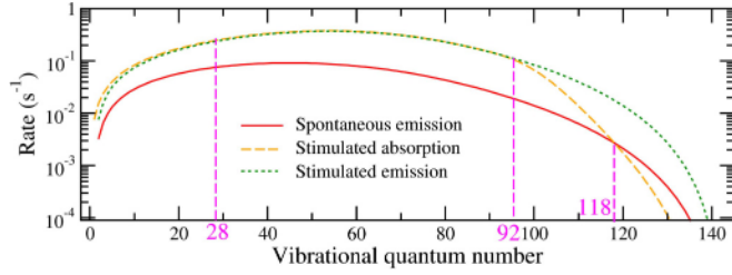
FIG. 6. Rates for spontaneous (stimulated) emission and absorption of the vibrational levels of the RbCa + X 1 Σ + ground state. The stimulated radiation rate is the sum of the absorption and stimulated emission rates. The vertical dashed line at v = 28 marks the photodissociation threshold for the 397 nm laser (see Sec. IV). At v = 92 , the absorption rate becomes smaller than the stimulated emission rate, and than the spontaneous emission rate at v = 118 .
