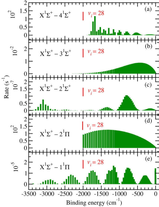
FIG. 8. Calculated photodissociation rates induced by the 397 nm cooling laser, assuming a laser intensity of I = 400 \text{mW}/\text{cm}^2 , as functions of the binding energy E_{v_i} of the X^1\Sigma^+ vibrational levels v_i , for the five open exit channels (a) 4^1\Sigma^+ , (b) 3^1\Sigma^+ , (c) 2^1\Sigma^+ , (d) 2^1\Pi , and (e) 1^1\Pi . The photodissociation threshold v_i = 28 is specified in red.
