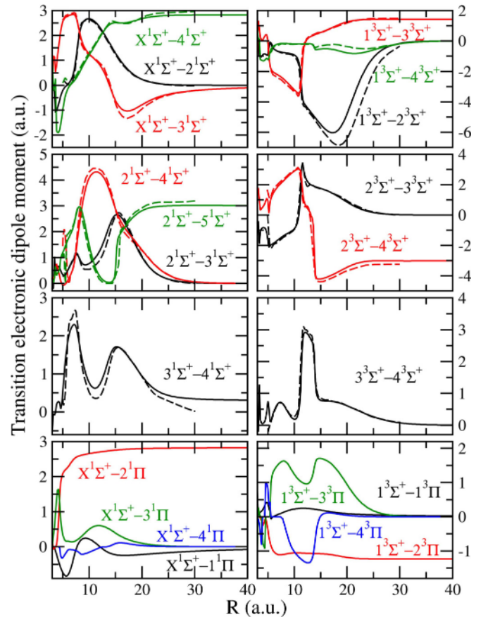
FIG. 14. Selected TEDMs computed in this paper (solid lines) compared to Ref. [29] (dashed lines).
