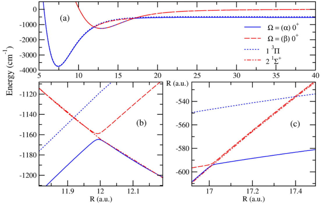
FIG. 9. (a) RbCa + Hund's case a 2^1\Sigma^+ and 1^3\Pi PECs and Hund's case c PECs labeled by (\alpha) and (\beta) for \Omega = 0^+ , (b) magnification around the crossing regions at R_1 = 11.9a_0 , and (c) at R_2 = 17.4a_0 .
