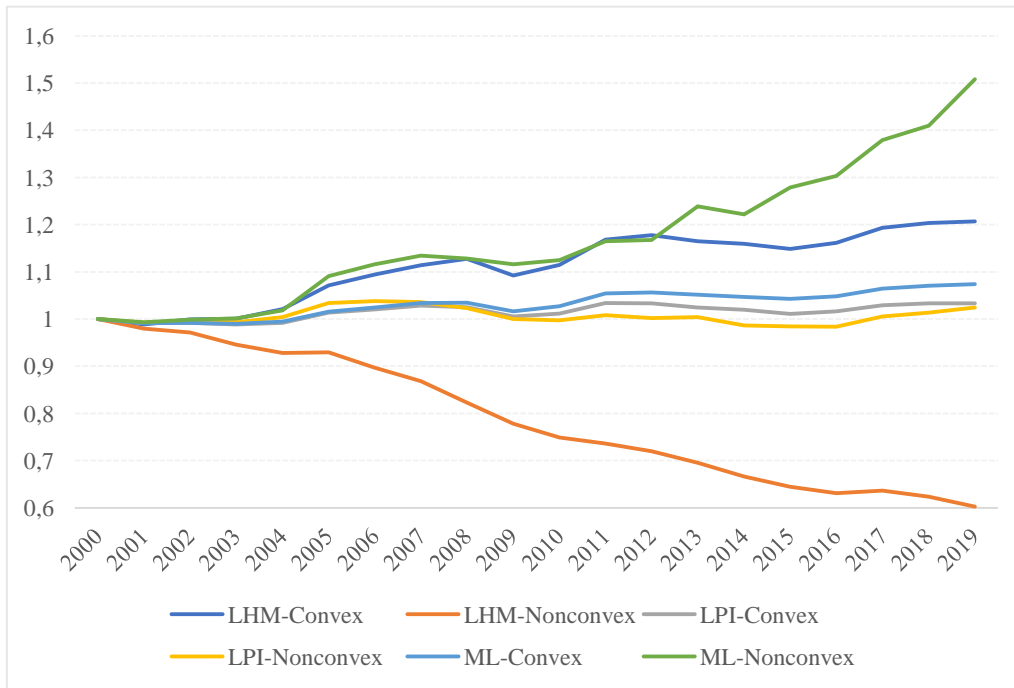
Fig. 3. Cumulative GTFP with the Luenberger-Hicks-Moorsteen, Luenberger productivity indicators, and Malmquist-Luenberger index under three group technologies and convexity and nonconvexity (2000-2019)
