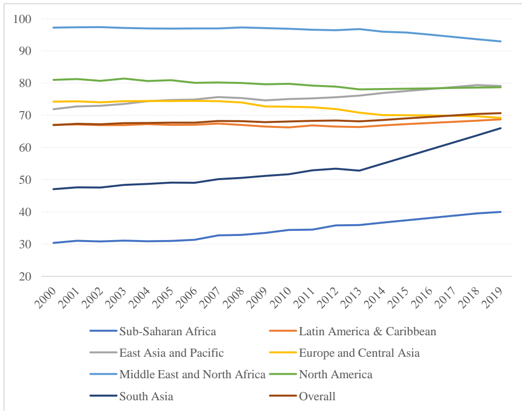
Fig. 2. Ratio of fossil fuel energy consumption in total energy use in different regions (2000-2019)
