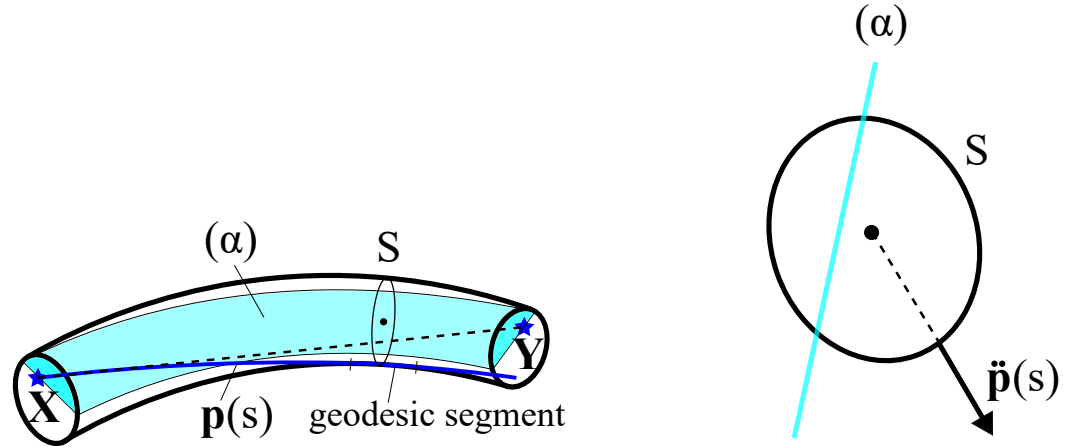
Figure 6. (Left) Tube portion between the cross-sections containing X and Y which can see each other. (\alpha) is an arbitrary plane containing XY but not containing \dot{p}(s_X) . The ESP p(s) only changes its direction \dot{p}(s) on its geodesic segment(s). S is an arbitrary cross-section of the tube where the geodesic segment crosses. (Right) On the projection view plane that is perpendicular to (\alpha) ( (\alpha) degenerates to a straight line), as \dot{p}(s) points outside the envelope of S , it also points away from (\alpha) . As \dot{p}(s_X) points away from (\alpha) , by mathematical induction \dot{p}(s) will point away from (\alpha) , \forall s \in [s_X, s_Y] .
