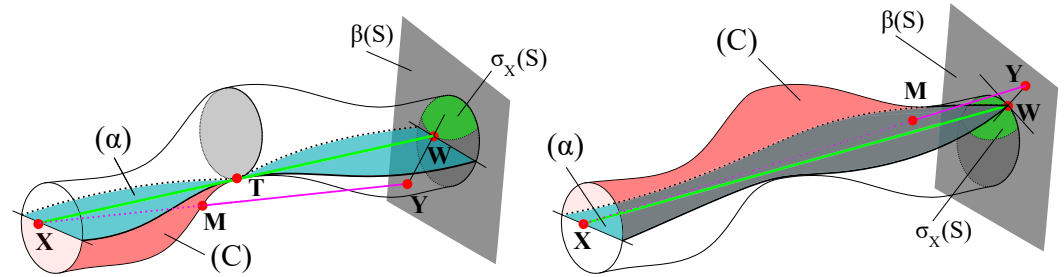
Figure 7. Point X can see cross-section S . Y be the intersection of the direction of the ESP \dot{p}(s_X) and the plane containing S . In \beta(S) and through Y , we draw an arbitrary straight line that intersects the visible area \sigma_X(S) . Let W be the intersection point that is closest to Y . (Left): W is in the inner zone of S . (Right): W is on the boundary of S .
