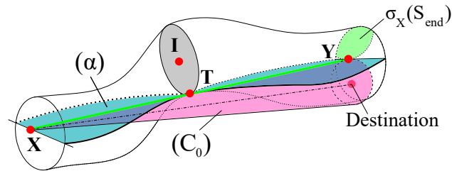
Figure A1. X can see the ending cross-section. By defining the cone surface (C_0) , we can prove that \Omega is coplanar with X, I, Y .
