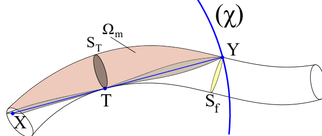
Figure A2. X cannot see the ending cross-section. It can see only one point Y on the furthest visible cross-section S_f .
