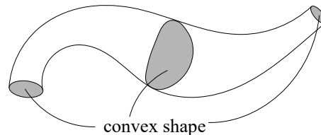
Figure 11. Canal space with convex and variable cross-sections.
