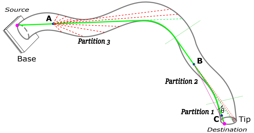
Figure 8. Three partitions of the shortest path corresponding to three sections of the tube. At \mathbf{A} belonging to \mathbf{P3} , the VP cannot see the ending cross-section S_{end} . The correct direction corresponds to the longest-length-of-sight. At \mathbf{B} belonging to \mathbf{P2} , it can see S_{end} , but not \Omega . The correct direction is towards the visible point \mathbf{Y} in S_{end} so that the angle \theta between \mathbf{BY} and \mathbf{B}\Omega is the smallest one. At \mathbf{C} in \mathbf{P1} , the particle can see \Omega . The correct direction is towards \Omega .
