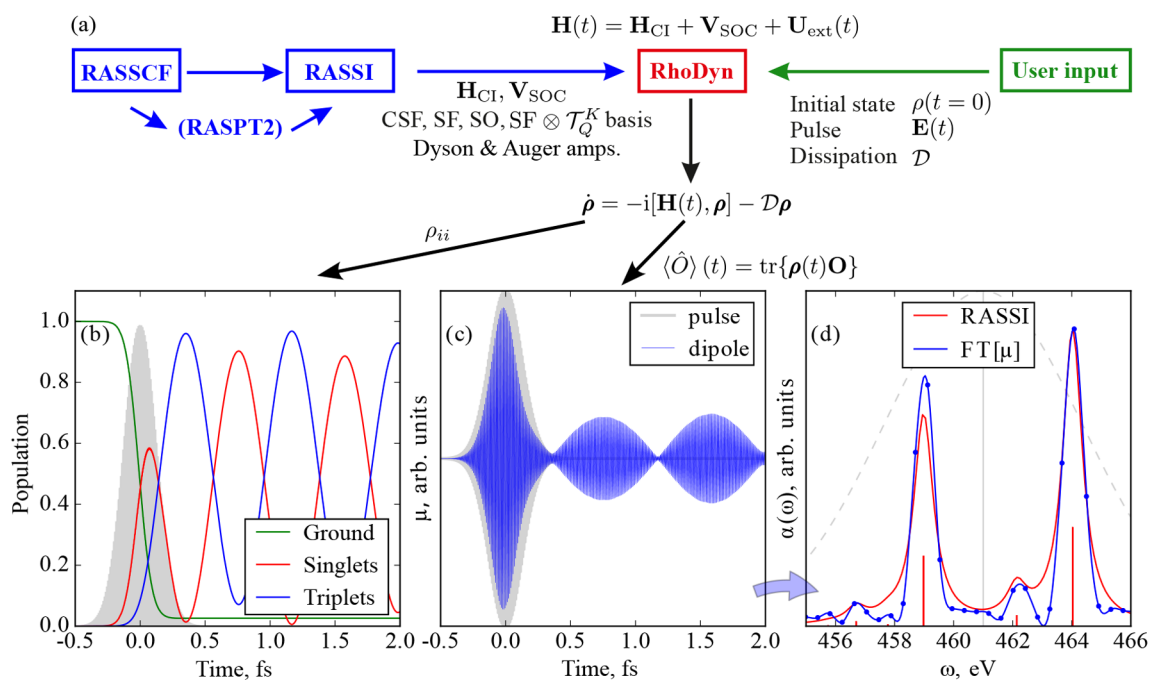
Figure 21. (a) Workflow and dependencies of the RhoDyn module. Here, H_{\text{CI}} , V_{\text{SOC}} , and U_{\text{ext}}(t) are the time-independent CI Hamiltonian responsible for electron correlation effects, SOC, and time-dependent external potential; for details, see ref 393. (b) Populations of ground, singlet, and triplet states of \text{TiCl}_4 molecule after the excitation with ultrashort X-ray pulse (pulse envelope shown as a shaded gray area). (c) Response of the dipole moment for the same case. (d) Linear XAS obtained as the Fourier transform of the dipole moment (pulse in energy domain shown as gray dashed line).
