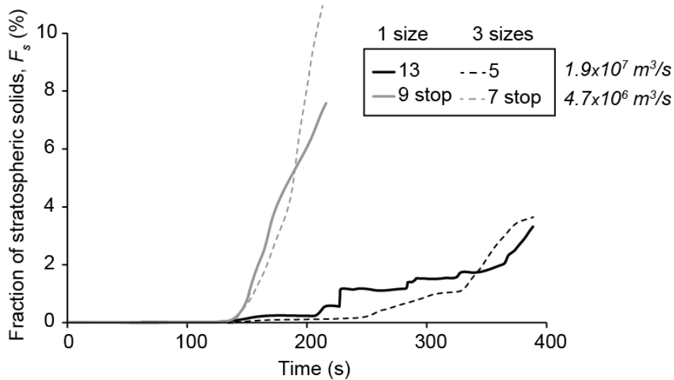
Figure 3: Temporal evolution of the fraction of solids injected into the stratosphere ( F_s ) for runs with one particle size (solid lines) and three particle sizes (dashed lines), respectively. Runs have the same volume flux (in italics) regardless of the number of particle sizes, but slightly different mass fluxes (see text). Black lines are runs continuously emitting ejecta and gray lines are runs that are stopped from emitting after 100 s.
