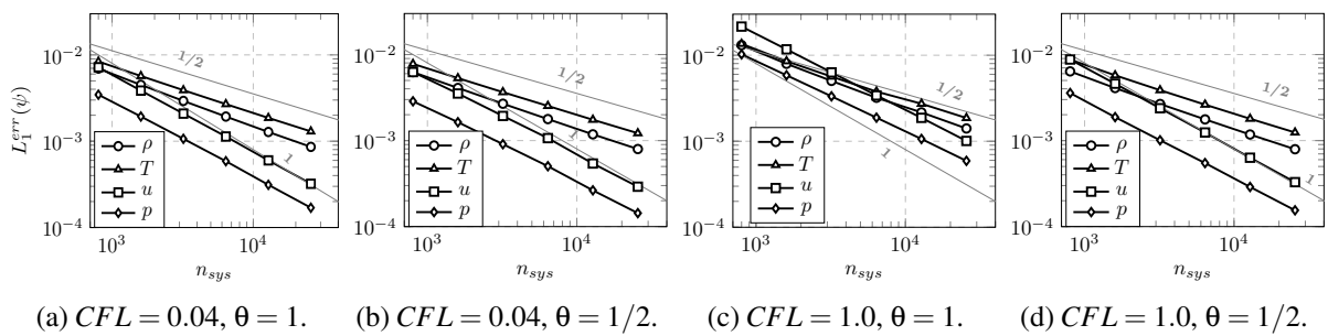
Figure 4: L_1 error convergence for the SOD case for two values of CFL and \theta .
