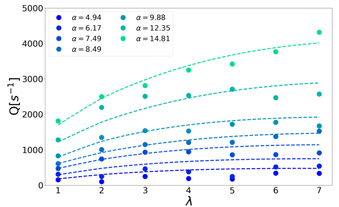
FIG. 10. Flow rate Q as a function of \lambda for various \alpha = D/\bar{d} . Dashed lines are the approximations given by Eq. (13) (see Sec. IV C).
