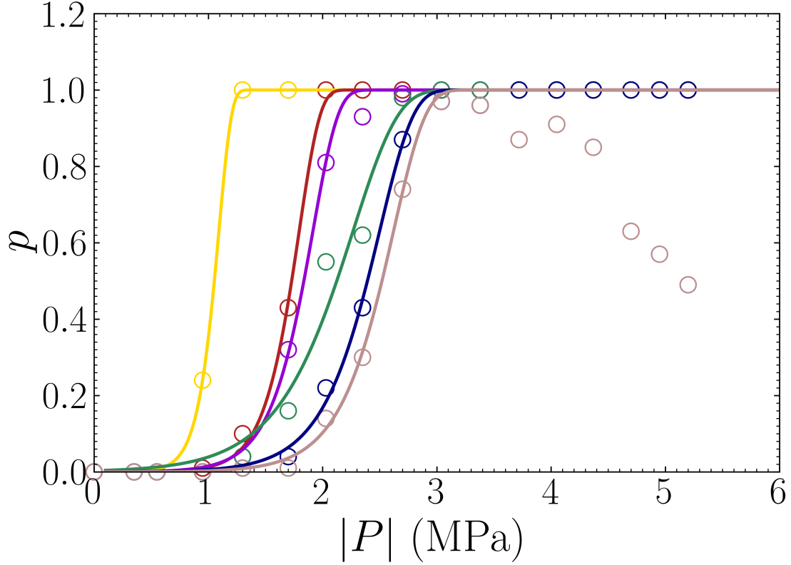
Figure 5: The probability p^{(n)} to detect an ADV event was evaluated as a function of the applied peak negative acoustic pressure P using different values for \zeta (3, 5, 6, 7, 9, and 10 from the left to the right probability curves). From the respective curves, we determined the following P_{0.5}^{(n)} values: 1.0, 1.7, 1.8, 2.1, and 2.4 MPa. The experiments were performed on a suspension of plain PFH droplets having a radius R = 20 \mu\text{m} , and at a droplet volume fraction \varphi_d = 5 \times 10^{-4} .
