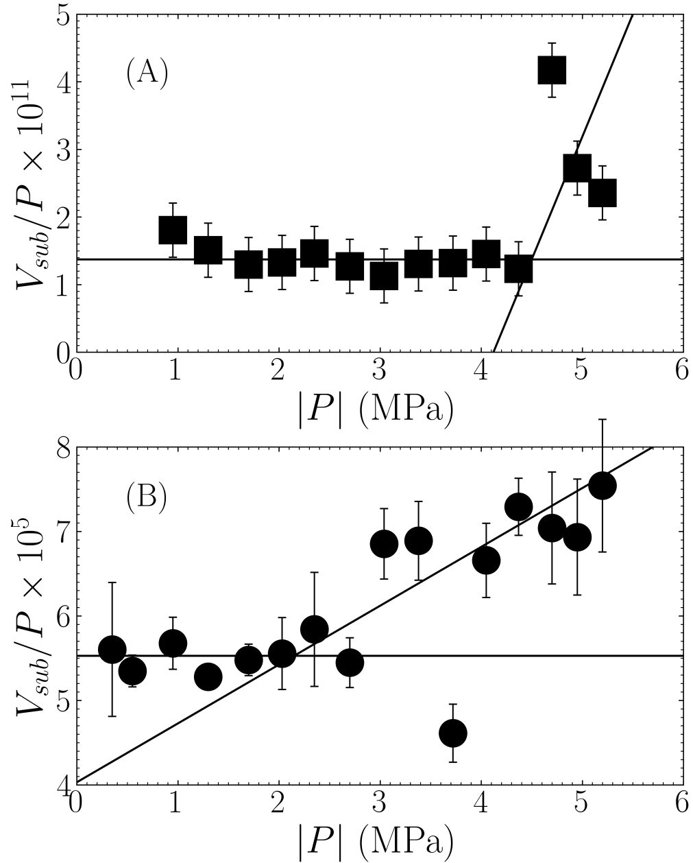
Figure 4: Normalized subharmonic component peak amplitude of the scattered response of a glycerol solution devoid of droplets (figure A) and of a suspension of PFH droplets ( R = 20 \mu\text{m} , \varphi_d = 5 \times 10^{-4} ) in glycerol (figure B) as a function of applied acoustic pressure P . The two lines intersect gives |P| = 4.5 \pm 0.3 MPa for the figure A and |P| = 2.1 \pm 0.3 MPa for the figure B. Consequently, the vaporization of PFH droplets appears before glycerol cavitation when pressure increases.
