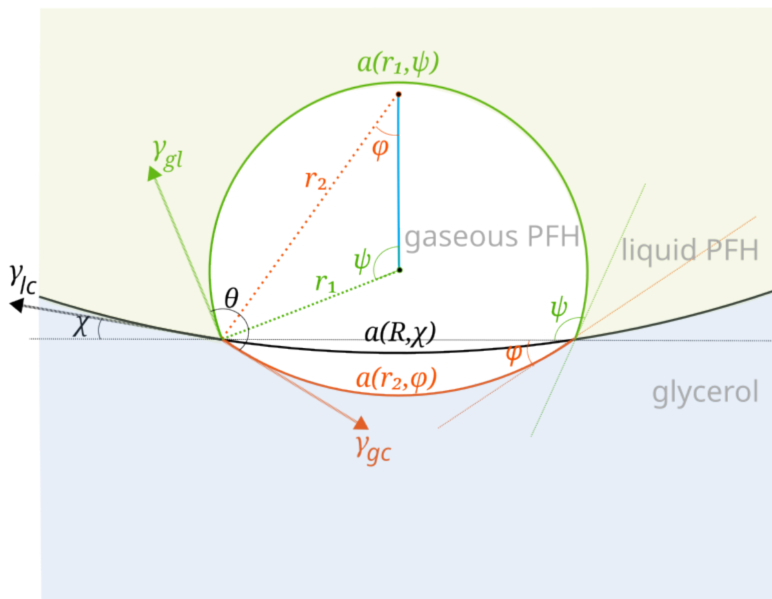
Figure 10: Schema of a nucleus on the surface of a plain PFH droplet surface (represented by the black solid line). The surface of the nucleus are represented by the green (with no surfactants) and orange (covered with surfactants) solid lines.
