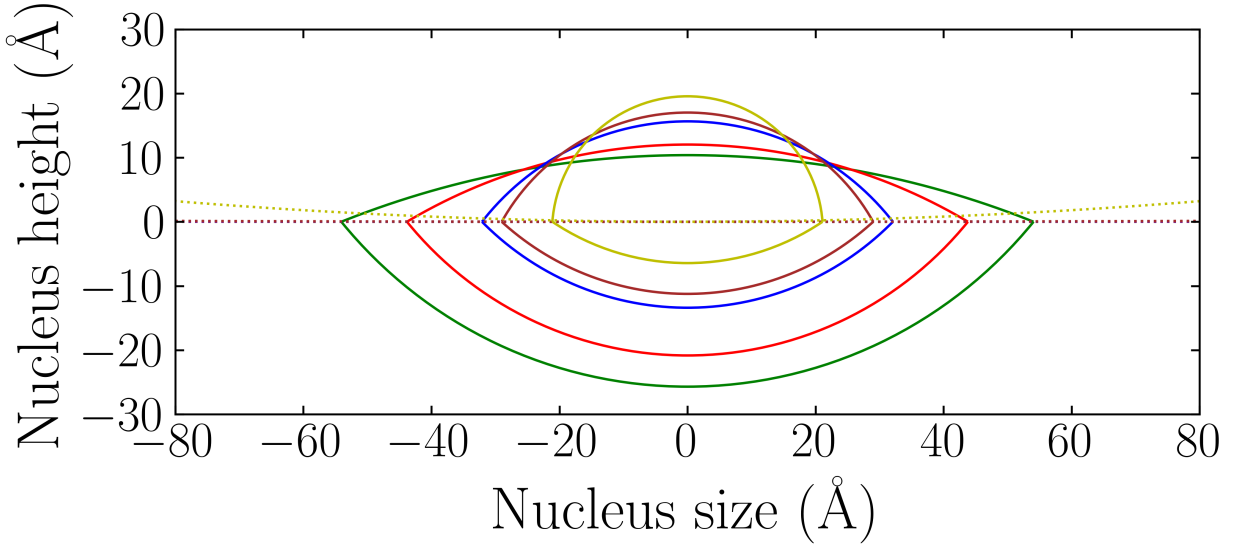
Figure 12: The figure displays the shape of the nucleus having radii r_1^* and r_2^* as showed by the solid lines. The dotted lines show the curvature of the droplet with radius R , where the liquid PFH is located on the top part of the graph. The nucleus size changes with the droplet radius R , where the colors green, red, blue, brown and yellow are for R = 30, 20, 5, 2.5, and 0.1 \mu\text{m} .
