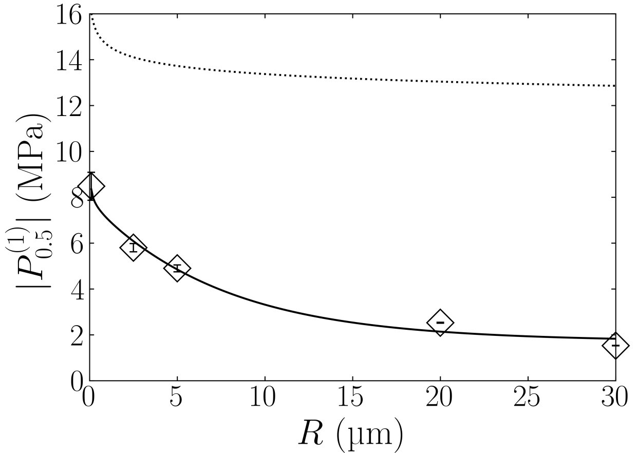
Figure 9: The diamonds are the values |P_{0.5}^{(1)}| previously given in Fig. 7. The dotted line represents the prediction of the homogeneous nucleation model. While the solid line is the prediction given by the heterogeneous nucleation model where \gamma_{gc} is the only unknown parameter, whose values are given in Fig. 11B.
