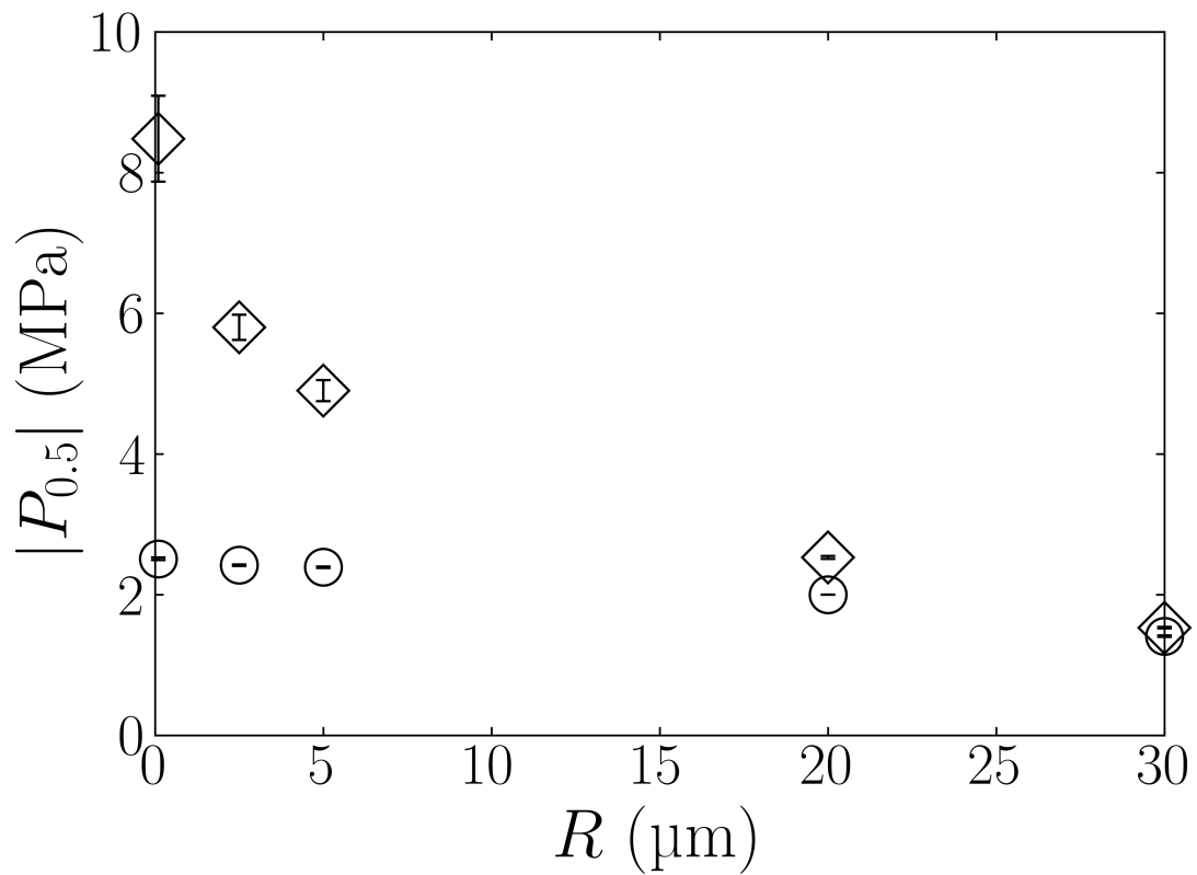
Figure 7: Values of |P_{0.5}^{(1)}| ( \diamond ) and |P_{0.5}^{(n)}| ( \circ ) determined for solutions at constant volume fraction of droplets ( \varphi_d = 5 \times 10^{-4} ), with droplet radius varying from 0.1 to 30 \mu\text{m} .
