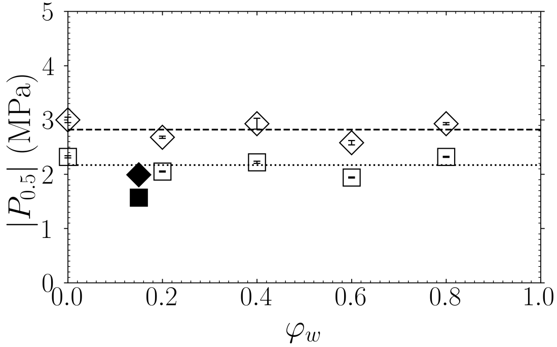
Figure 8: The squares represent the values of |P_{0.5}^{(n)}| for a suspension of either water multi-core PFH droplets ( \square ) or water single-core PFH droplets ( \blacksquare ). While the lozenges represent the values of |P_{0.5}^{(1)}| for a suspension of either water multi-core PFH droplets ( \diamond ) or water single-core PFH droplets ( \blacklozenge ). All suspensions contain an identical droplet volume fraction of \varphi_d = 5 \times 10^{-4} and an identical radius of R = 20 \mu\text{m} . The water droplets are stabilized by Krytox 157 FSL and possess a radius of either R_w = 10.5 \mu\text{m} or 250 \text{nm} when a PFH droplet contains, respectively, a single water droplet ( \blacksquare and \blacklozenge ) or many of them ( \square and \diamond ).
