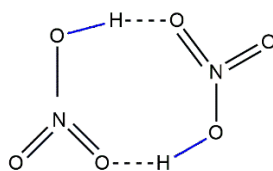
Fig 2. Schematic representation of the molecular structure of nitric acid in aqueous medium.
