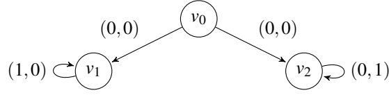
Figure 12.7: Randomised strategies are needed to achieve any percentile query of the form \mathbb{P}_{\mathcal{D},v_0}^\sigma[\text{MeanPayoff}_1^- \geq 1] \geq \mu_1 \wedge \mathbb{P}_{\mathcal{D},v_0}^\sigma[\text{MeanPayoff}_2^- \geq 1] \geq \mu_2 with \mu_1, \mu_2 > 0 .
