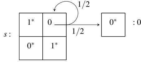
Figure 7.2: Concurrent discounted game with value v_s = -2 + \sqrt{4 + 2(1 - \gamma)}
