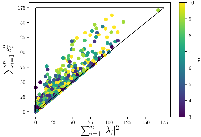
Figure S1.1: Test of conjecture 4: for a wide array of randomly generated matrices of size n \times n with n = 3, \dots, 10 . We could never find any matrix for which the inequality \sum_{i=1}^n |\lambda_i|^2 \leq \sum_{i=1}^n s_i^2 (and we know it holds for n = 2 ).
