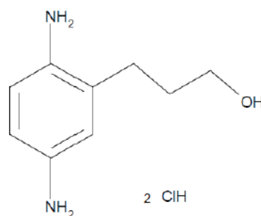
Dihydrochloride salt
