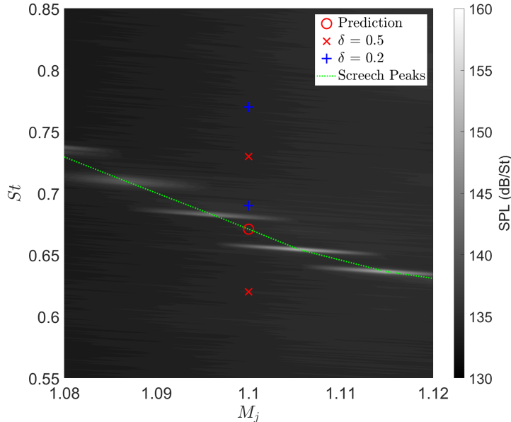
Figure 22: Sound pressure levels (dB/St) measured for the twin-jet system running at several M_j for S = 2 . A line highlighting the A1 screech peaks is included. The k_p^-(0, 2) branch and saddle points are computed at M_j = 1.1 for the SA symmetry using a \delta of 0.2 (+), and 0.5 (x) respectively. A screech frequency prediction using the finite-thickness model is shown (○), with the KH and k_p^- wavenumbers computed using \delta of 0.2 and 0.5 respectively. Parameters used for this prediction are, s = 4 , p = 4 and \phi = 0 .
