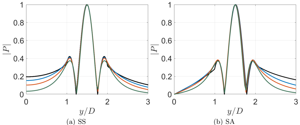
Figure 9: Absolute value of normalised k_p^-(0,2) pressure eigenfunctions along the y axis for both vortex-sheet model and varying velocity profiles in finite thickness model. M_j = 1.16 , S = 3 and St = 0.67 . Only one jet is shown for both the inter-jet ( y/D < 1 ), inner ( 1 < y/D < 2 ), and outer ( y/D > 2 ) regions. For (a) SS and (b) SA. Vortex sheet (Black), \delta = 0.12 (blue), \delta = 0.2 (red) and \delta = 0.4 (green)
