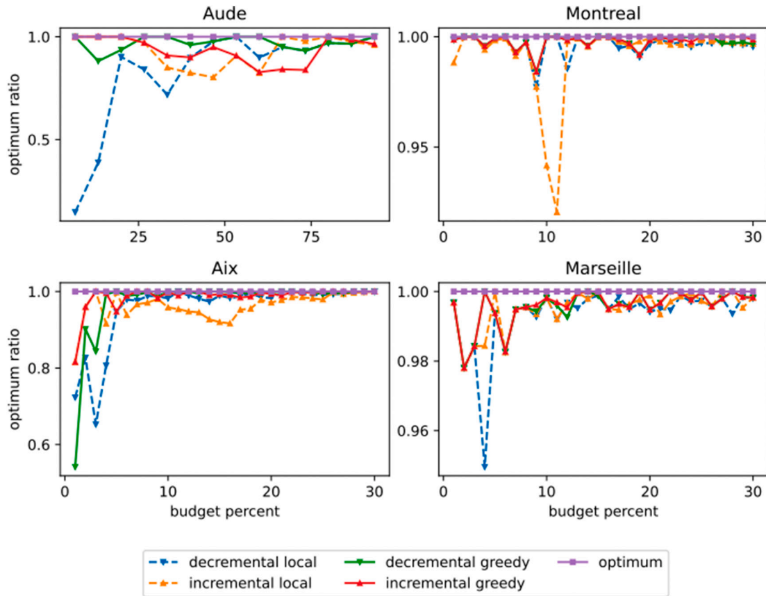
Fig. 3. Percentage gain in ECA achieved by the solutions of the different algorithms compared to the optimal solution (Hamonnic et al., 2023) as a function of the budget.
