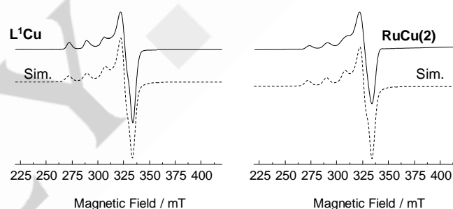
Figure 3. X-band CW-EPR spectra recorded for 1 mM acetonitrile solutions of L 1 Cu and RuCu(2) (solid lines) with simulations (dashed lines). Acquisition parameters: temperature = 25 K; MW frequency = 9.388 GHz ( L 1 Cu ), and 9.636 GHz ( RuCu(2) ); MW power = 20 \mu W; modulation amplitude = 1.0 mT; conversion time = 163.84 ms.
