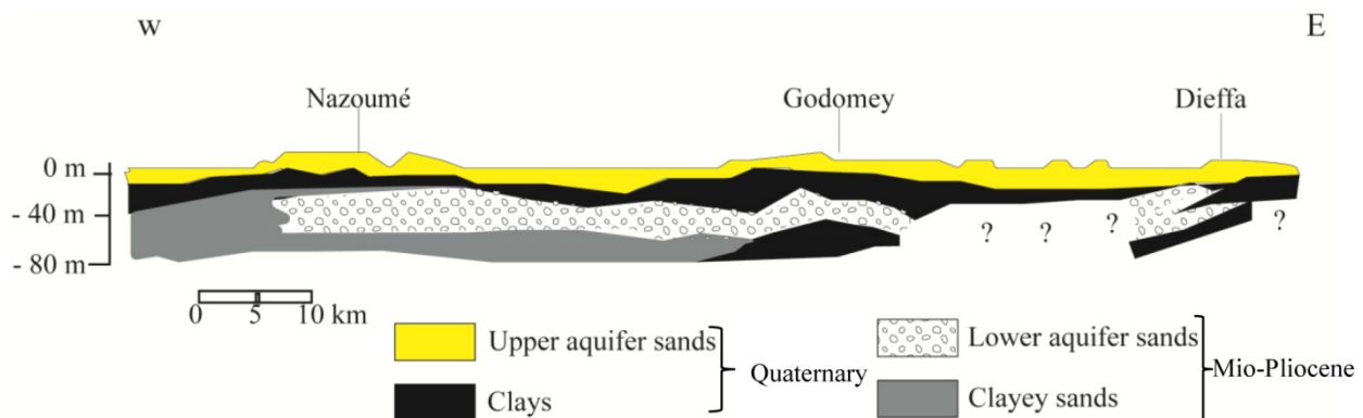
Figure 3. West–East geological cross section along the coastal plain of Benin [20,21,26]. Question marks indicate levels or depths with no available data or references. Vertical axis is in meters above sea level.
