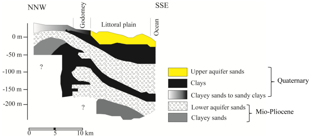
Figure 2. Longitudinal NNW-SSE geological cross section of the coastal sedimentary basin of Benin (modified from [21]). Question marks indicate levels or depths with no available data or references. Vertical axis is in meters above sea level (m asl).
