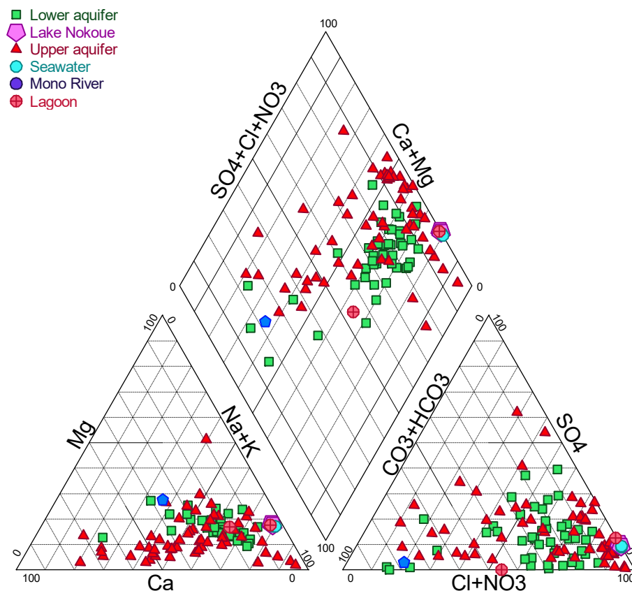
Figure 4. Piper diagram of coastal groundwater in Benin. The chemical composition of seawater, Mono River, Lake Nokoué, and lagoons are also plotted.
