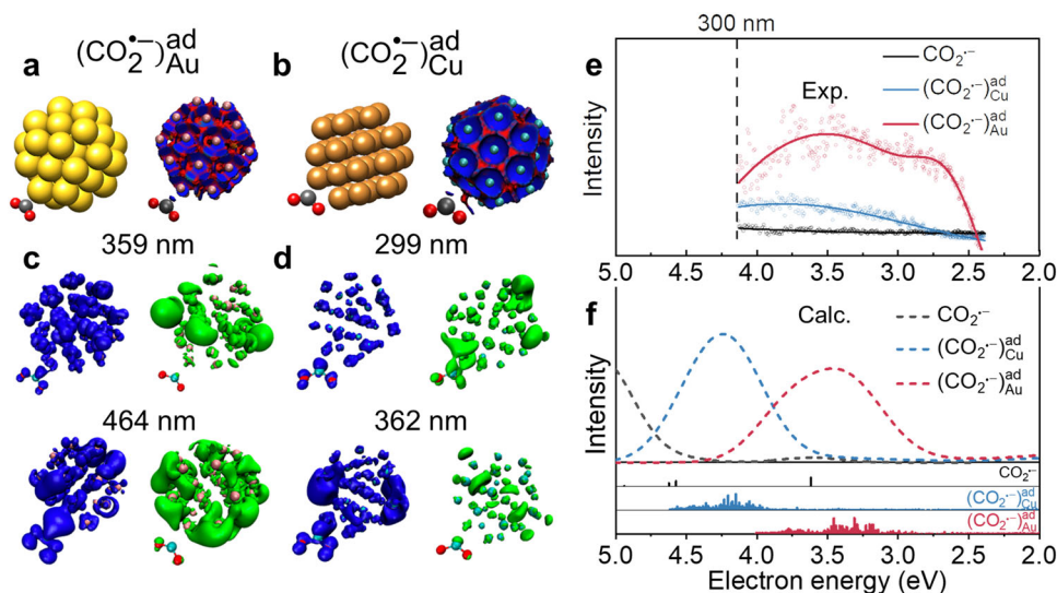
Fig. 4 | The simulation of \text{CO}_2^{\cdot-} radical stabilized on metal nanocatalysts.
