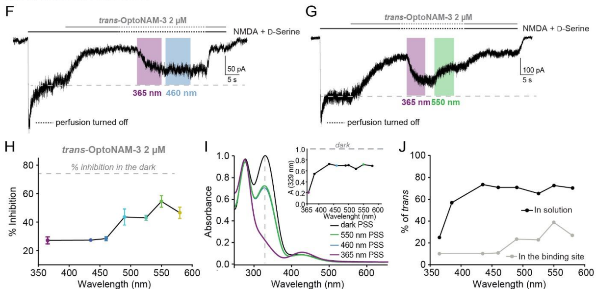
Fig. 4. Binding of OptoNAM-3 onto GluN1/GluN2B NMDARs changes its photochemical properties. (A-E) Spectral properties of trans to cis isomerization (A, B) Current traces from DIV 6-8 cultured cortical neurons following application of NMDA (300 \mu M) and D-serine (50 \mu M), as well as 2 \mu M OptoNAM-3. As described in Fig. 3, once steady-state inhibition by trans -OptoNAM-3 was reached, the patched cell and the surrounding extracellular medium were illuminated by various wavelengths: in our example 460 nm (blue bar) in (A) and 550 nm (green bar) in (B) followed by 365 nm (violet bar) as a control for the lowest amount of inhibition. (C) Percentage of inhibition by 2 \mu M OptoNAM-3 upon shining different wavelengths on the cell. 365 nm was the most efficient wavelength allowing reduction of inhibition to 27 \pm 2.5\% . n = 23 for 365 nm; n=4 for 435 nm; n=5 for 490 and 550 nm; n=6 for 460 and 525 nm. Data points from 435 and 580 nm represented in this figure were scaled between 365 nm and dark condition for better accuracy (see Method for calculation protocol). (D) UV-visible spectra of a solution of OptoNAM-3 in the dark (black curve) and after illumination with 365, 460 or 550 nm (violet, blue and green curves, respectively). Inset, absorbance at the peak absorbance wavelength of the dark state (329 nm) of OptoNAM-3 following illumination at various wavelengths of the dark PSS. Note that in solution, the
