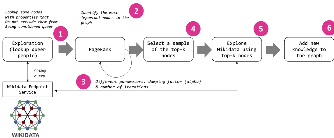
Figure 3: Crawled method pipelines
