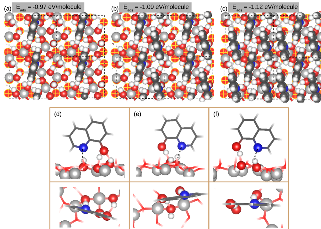
Fig. 4 Top views of the most stable adsorption configurations of the native 8-HQ molecules on the \gamma - \text{Al}_2\text{O}_3(111)/\text{Al}(111) surface, with their adsorption energies (PBE-D2 approach). Snapshots (a–c) correspond to surface coverages of 1.18, 2.36 and 3.54 molecule \text{nm}^{-2} , respectively. Snapshots (d–f) illustrate side and top views for the different adsorption features of the species.
