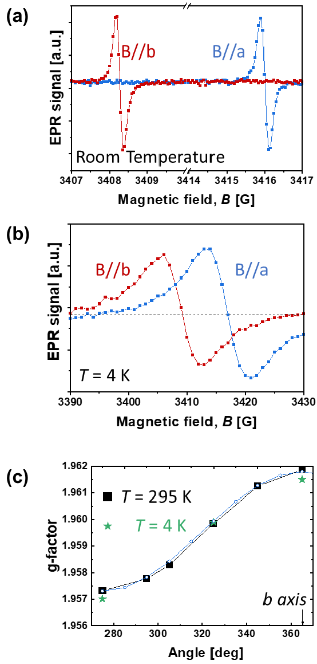
Figure 2. (a) SD EPR spectra at room temperature for B//b and B//a , (b) at T=4 K; (c) angular variation of the spin S = 1/2 spectrum g -values, which identifies it as a shallow donor
