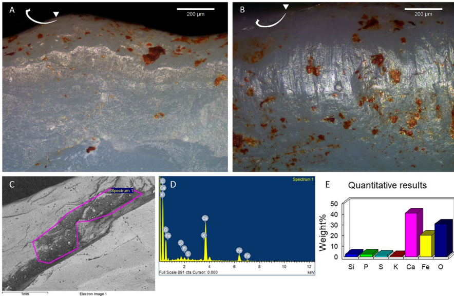
Fig. 13 A, B Use-wear produced by the hard nodule of haematite (ochre), 10 min (ref. CU.05) (at 100×). C One of the two sampling areas selected for residue analysis on CU.05 (image by scanning electron microscopy). D Energy-dispersive X-ray spectroscopy (EDX) spectrum E Bar chart of the elemental composition performed on the selected sampling area
