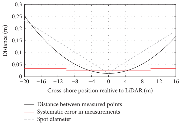
FIGURE 3: Distance between the points measured by the TLS (black line), for this experimental setup described in this paper. This value evolves from 0.014 m at the Nadir to 0.25 m at the most seaward captured location. The systematic error and the spot diameter provided by the manufacturer are also plotted (red continuous and grey dashed lines resp.).
