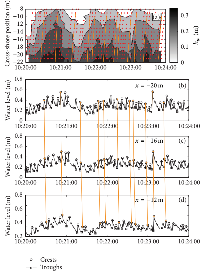
FIGURE 5: Example showing the wave extraction method in the inner surf zone. The wave-period-averaged water depth h_w contours are shown in (a), where red dots represent the detected wave crests. The orange lines are the waves selected in this time window for the celerity calculations. Panels (b), (c), and (d) represent the water surface elevations at three cross-shore locations, with the chosen waves tracked across them. Extracted wave crests and troughs are represented by black circles and squares, respectively.
