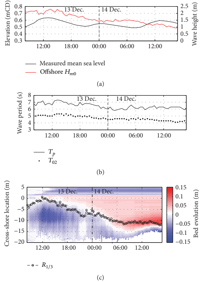
FIGURE 6: Bed extraction results: (a) measured mean water levels above Chart Datum at Fos-sur-Mer port and offshore significant wave height measured by a buoy close to Sete; (b) measured wave periods ( T_p and T_{02} ) by the same buoy; (c) beach morphological evolution for the 13th and 14th of December (30 continuous hours of measurement). Erosion and accretion patterns were calculated by subtracting the initial beach profile to that of the actual moment. Red color corresponds to accretion while blue corresponds to erosion. The significant run-up limit R_{1/3} is shown as a circled black line.
