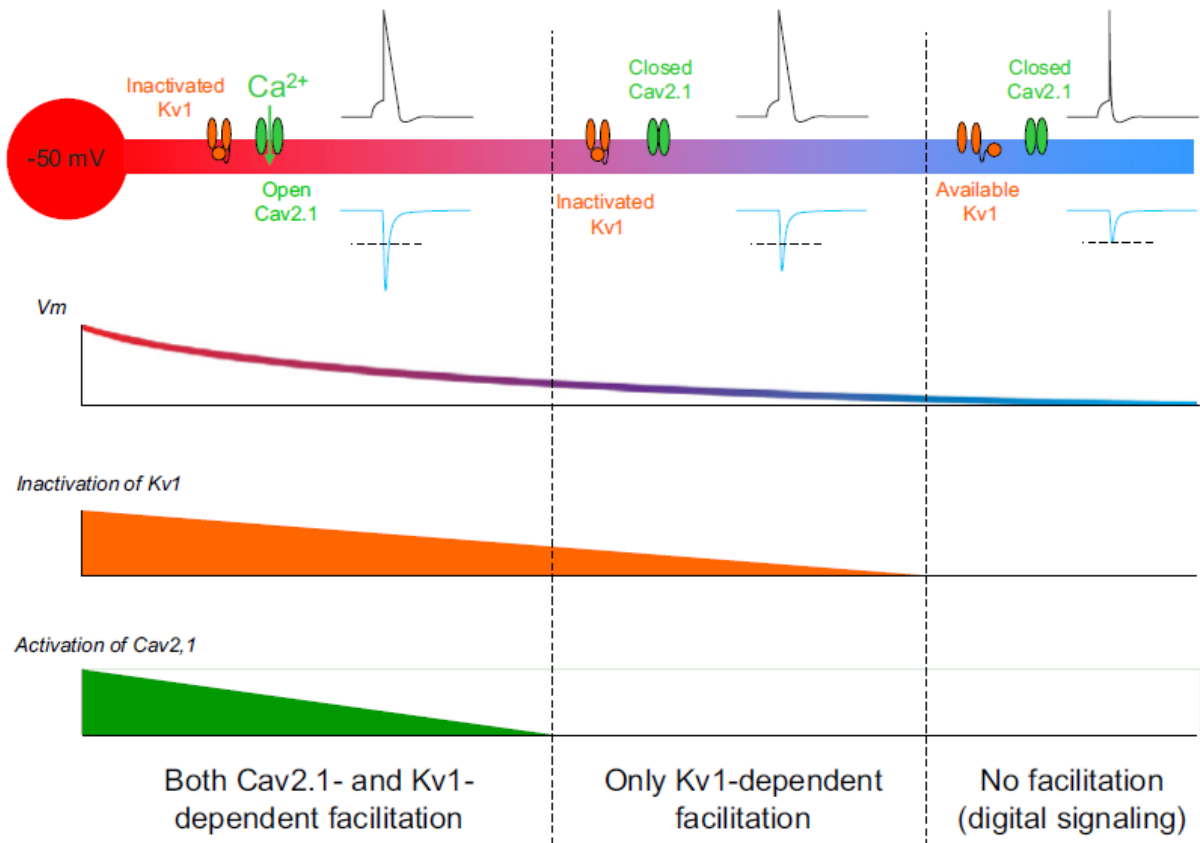
Fig. 5. Spatial extent of Kv1- and Ca 2.1 -dependent AD facilitation. In the proximal part of the axon, the depolarization is sufficient for inactivating Kv1 channels and activating Cav2.1 channels, resulting in a maximal AD facilitation (Kv1- and Cav2.1-dependent ADF). In the medial part of the axon, the depolarization is sufficient to inactivate Kv1 channels but cannot activate Cav2.1. In this region, only Kv1-dependent facilitation is observed. In the distal part of the axon, the depolarization originating in the soma is too small to inactivate Kv1 channels and no facilitation occurs.
