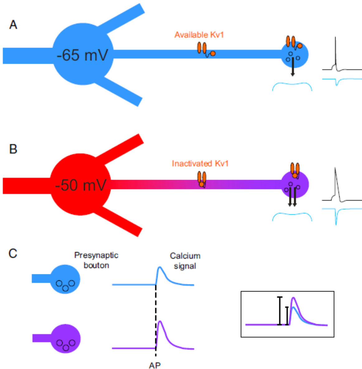
Fig. 3. Kv1-dependent analog-digital facilitation. A. With digital-only signaling the neuronal membrane voltage ( V_m ) is held at -65\text{ mV} , Kv1 channels remain available, resulting in a rapid termination of the spike response. B. Analog subthreshold depolarization ( -50\text{ mV} at the soma) propagates from the somatic compartment and along the axon to the terminal, resulting in inactivation of Kv1 channels. This produces a broadening of the action potential and results in enhanced spike-evoked \text{Ca}^{2+} entry and incremented neurotransmitter release. C. Calcium signals produced by the spike in the digital-only signaling (blue) or in the analog-digital signaling (purple). Note the increased amplitude of the spike-evoked calcium transient (inset).
