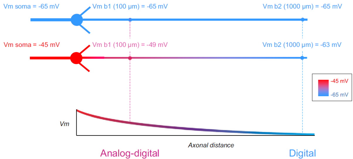
Fig. 2. Voltage decay along axons. Top, voltage distribution when the neuron is at rest ( -65 mV). The voltage is constant in the soma, in the proximal presynaptic bouton (b1, 100 \mu m from the soma) and in the distal bouton (b2, 1000 \mu m from the soma). When the cell body is depolarized, ( -45 mV) voltage drops along the axon because of cable properties. Bottom, voltage ( V_m ) decay along the axon. Note that AD transmission is restricted to proximal presynaptic bouton (b1), whereas pure digital transmission occurs at distal bouton (b2).
