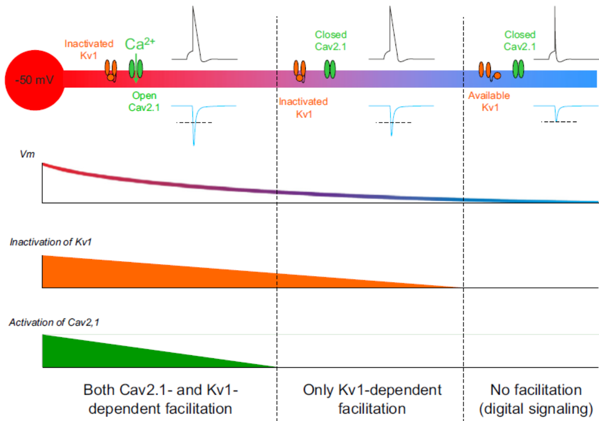
Fig. 5. Spatial extent of Kv1- and Ca2.1-dependent AD facilitation. In the proximal part of the axon, the depolarization is sufficient for inactivating Kv1 channels and activating Cav2.1 channels, resulting in a maximal AD facilitation (Kv1- and Cav2.1-dependent ADF). In the medial part of the axon, the depolarization is sufficient to inactivate Kv1 channels but cannot activate Cav2.1. In this region, only Kv1-dependent facilitation is observed. In the distal part of the axon, the depolarization originating in the soma is too small to inactivate Kv1 channels and no facilitation occurs.
