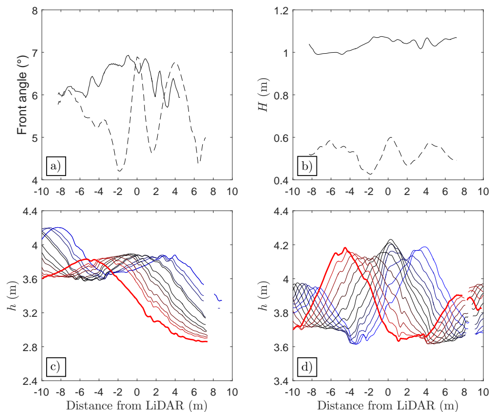
Figure 7. Spatial evolution of waves numbers 1 and 2 (see Figure 4). (a,b) show the wave front angle and height, respectively, for wave 1 (black continuous line) and wave 2 (black dashed line); (c,d) show the wave propagation of waves 1 and 2, respectively: the wave profile is shown when the crest is detected at 0.7 m intervals. For clarity, each profile is drawn in a different colour: wave profiles are first shown as thick red lines (first profile shown as thick red lines) and evolve towards black at the nadir, and finally blue after having passed under the LiDAR. Note that the tidal bore propagates from left to right (axis positive in the upstream direction).
