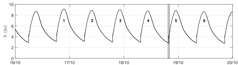
Figure 2. Water depth evolution over the course of the experiments. The water depth was derived from the pressure measurements assuming hydrostatic pressure (Equation (1)). The present paper uses mainly data from the tide monitored number 5, which is highlighted by the grey region.
