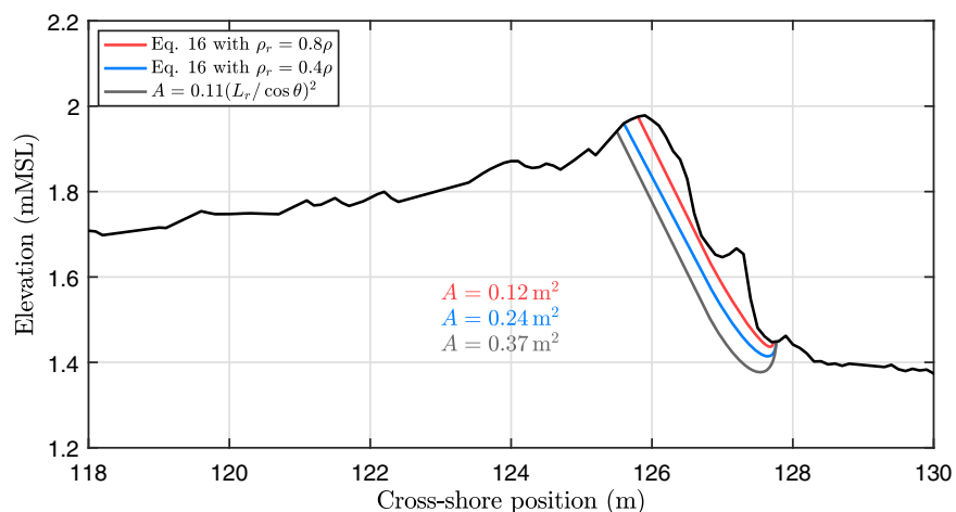
Figure 7. Surface roller areas shown under an example wave profile (fourth wave of the group, see Appendix A). To facilitate the calculation of the roller area, the interface between the roller and the wave was assumed to have an ellipsoidal shape close to the roller toe.
