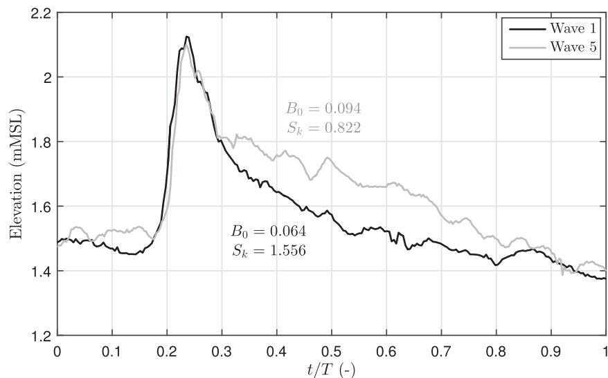
Figure A2. Temporal wave profile at x = 130 m of the individual wave numbers 1 and 5 of the wave group from Figure A1a.
