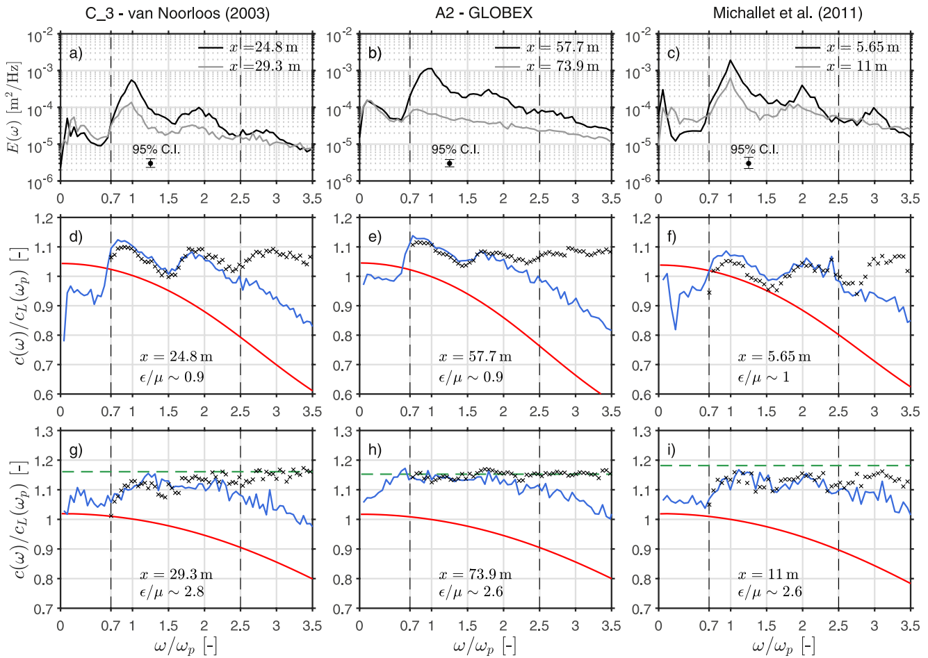
Figure 3. Assessment of the Boussinesq theory (Equation 2) to predict wave phase spectra for the experiments of van Noorloos (2003, left panels), GLOBEX (middle panels) and Michallet et al. (2011, right panels). Panels (a–c) show the energy density spectra of \zeta at two positions corresponding to shoaling panels (d–f) and breaking situations panels (g–i). The normalized wave phase velocities predicted with the Boussinesq (blue lines) and linear wave (red line) theories are compared against observations (black crosses). In the surf zone panels (g–i), the green horizontal line corresponds to the modified shallow-water wave celerity predictor ( \sqrt{gh(1+\epsilon)} ). The cross-shore locations were selected based on the Ursell number ( U_r \sim 1 and U_r \sim 2.6 – 2.8 for shoaling and breaking situations, respectively) and are indicated for each experiment. The vertical lines indicate the range of frequencies [0.7\omega_p; 2.5\omega_p] used for the depth-inversion.
