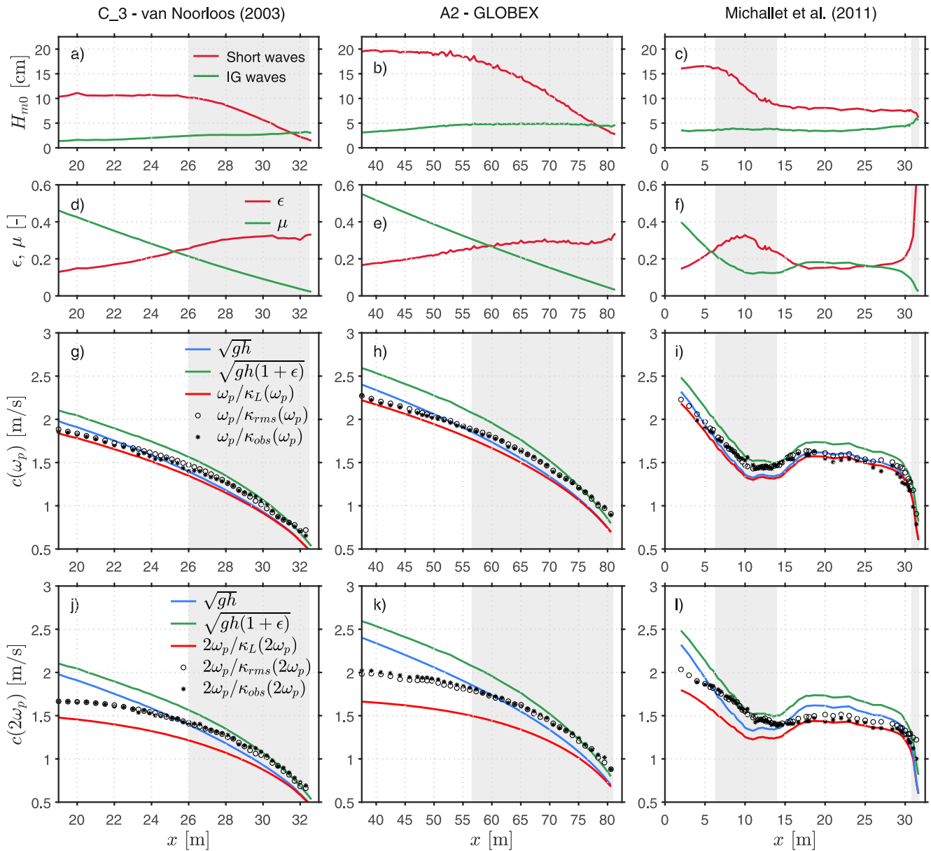
Figure 2. Assessment of the Boussinesq theory (Equation 2) to predict the cross-shore evolution of dispersive properties during the experiments of van Noorloos (2003, left panels), GLOBEX (middle panels) and Michallet et al. (2011, right panels). Panels (a–c) show the cross-shore evolution of significant wave height H_{m0} for short and infragravity (IG) waves computed as (16\zeta^2)^{1/2} (cutoff frequency at 0.6f_p ). Panel (d–f) show the amplitude ( \epsilon = H_{m0}/2h ) and dispersion ( \mu = (\kappa_p h)^2 ) parameters. Panels (g–j) show the observed and Boussinesq predictions of the wave phase velocity at the peak frequency \omega_p , while panels (k–m) show those at the second harmonic 2\omega_p . These quantities are compared with the predictions from the linear wave dispersion (Equation 1) and shallow-water predictors. In all panels, the gray shaded area indicates regions of the wave flume where wave breaking occurs.
