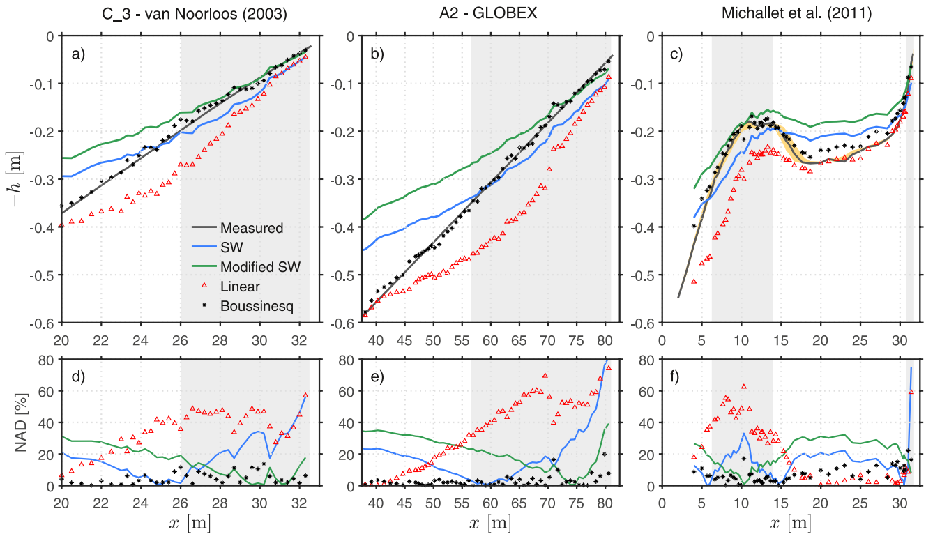
Figure 4. Results of the depth inversion applications for the experiments of van Noorloos (2003, left panels), GLOBEX (middle panels) and Michallet et al. (2011, right panels). Panels (a–c) show the beach elevation profile estimated using Boussinesq (Equation 6) and the linear wave theory (Equation 7). These are compared with estimates based on shallow-water waves propagation velocity (“SW”: c_{bulk} \sim \sqrt{gh} and “Modified SW”: c_{bulk} \sim \sqrt{gh(1 + \epsilon)} ). In panel (c), the orange-shaded area around the measured profile corresponds to the bed elevation changes observed during the considered wave sequence. Panels (d–f) show the corresponding normalized absolute difference (NAD) of measured and predicted water depths. In all panels, the gray shaded area indicates regions of the wave flume where wave breaking occurs.
