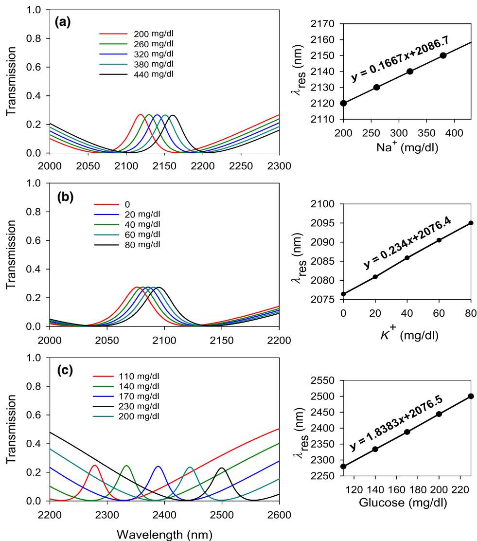
FIG. 8. Transmission spectra versus the wavelength for different concentration C of (a) \text{Na}^+ , (b) \text{K}^+ , and (c) glucose solution. Change of the peaks' wavelength versus the concentrations are presented in the insets of (a),(b),(c), respectively.
