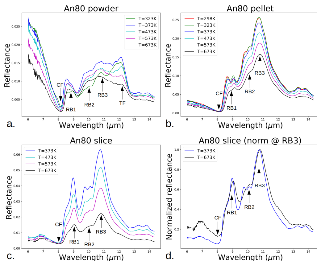
Figure 9. MIR spectra of the samples of plagioclase at different temperatures. (a) powder; (b) pellet; (c) slice; (d) slice at T = 373\text{ K} ( 100\text{ }^{\circ}\text{C} ) and 673\text{ K} ( 400\text{ }^{\circ}\text{C} ) normalized to the RB3 maximum. The approximate positions of CF, RB1, RB2, RB3, and TF are indicated on each panel.
