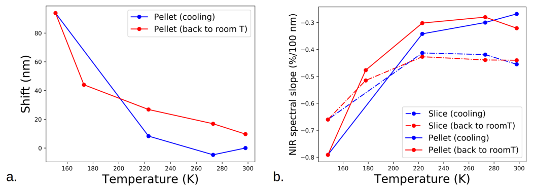
Figure 8. (a) Shift in the 3.0 μm band with respect to temperature for the pellet of plagioclase; (b) NIR spectral slope on 1.7–2.6 μm with respect to the temperature for the slice and pellet of plagioclase.
