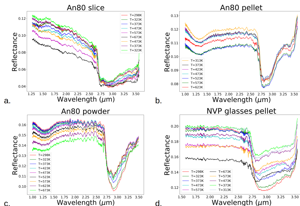
Figure 3. NIR spectra of plagioclase samples and volcanic glasses at different temperatures for the heating experiment. (a) slice of plagioclase; (b) pellet of plagioclase; (c) powder of plagioclase; (d) pellet of volcanic glasses.
