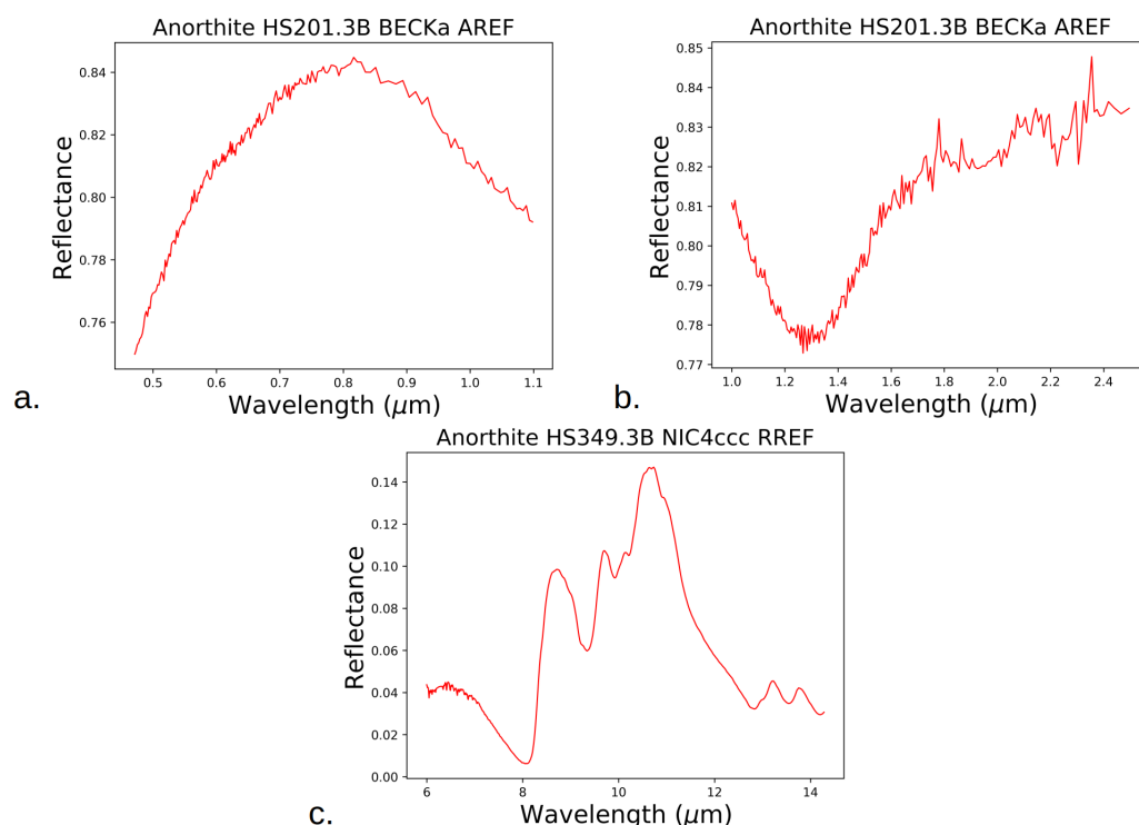
Figure A1. Spectra of two anorthite samples from the USGS spectral library. The spectra were restricted to the wavelengths used for our measurements for better comparison. (a) VNIR range (0.47–1.1 μm); (b) NIR range (1.0–3.5 μm, but data are only available on 1.0–2.5 μm); (c) MIR range (6.0–14.3 μm).
