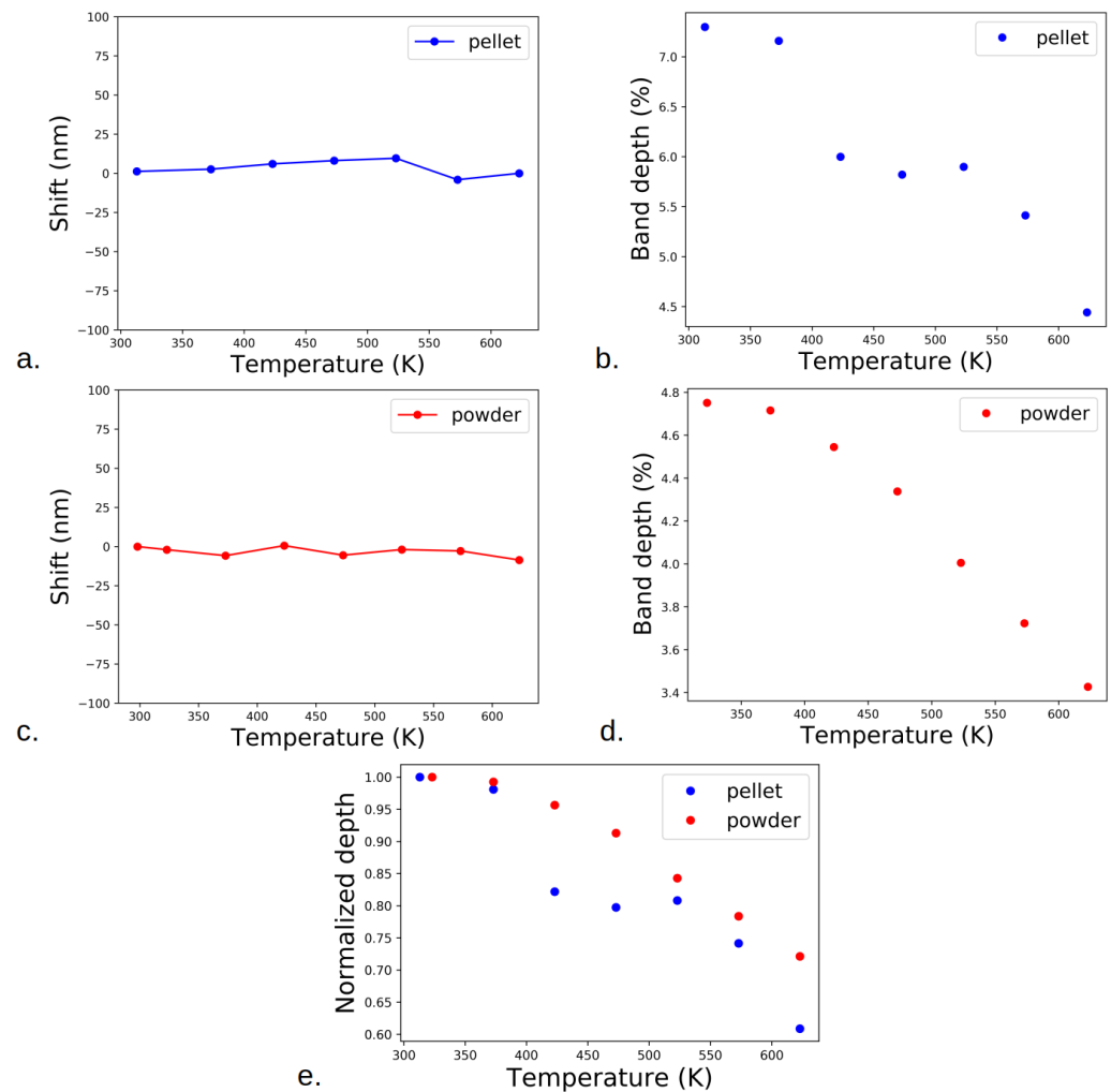
Figure 4. Spectral variations in the 1.3\text{ }\mu\text{m} band with respect to temperature for the pellet ((a) shift; (b) depth) and the powder of plagioclase ((c) shift; (d) depth); (e) depths normalized to the lowest available temperature value (313 K [ 40\text{ }^{\circ}\text{C} ] for the pellet, 323 K [ 50\text{ }^{\circ}\text{C} ] for the powder).
