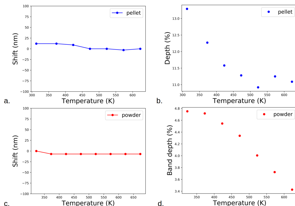
Figure 5. Spectral variations in the 3.0 μm band with respect to temperature for the pellet ((a) shift; (b) depth) and the powder of plagioclase ((c) shift; (d) depth).
