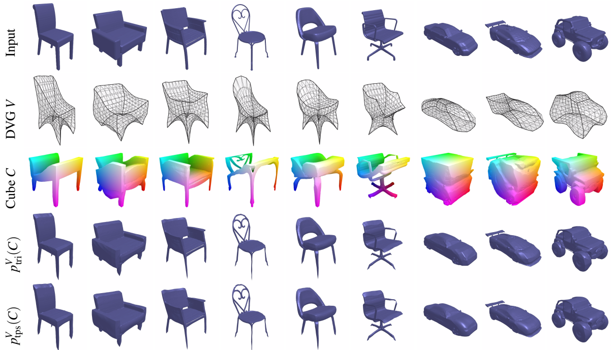
Figure 4: (Zoom in to see details) Qualitative results for shape reconstruction via DVGs: estimating V for each shape allows to cubify it ( C ), and this can be reprojected into V by a trilinear p_{\text{tri}}^V or a spline p_{\text{tps}}^V projector (see 3.1), the latter yielding smoother surfaces. The cubified shapes are color-coded by assigning a value in [0, 1]^3 to an RGB color.
