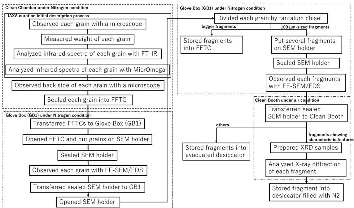
Fig. 2 Flowchart of a series of processes for JAXA-DD samples. Note that the majority of grains have only been exposed to vacuum and nitrogen environment in clean chamber and glove box, and then have been stored under nitrogen environment
