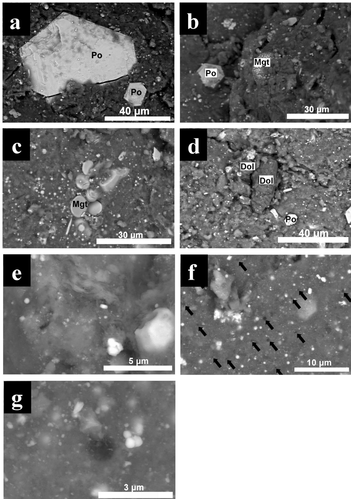
Fig. 4 Back-scattered electron images of major constituent phases in A0042, dark group. a Euhedral hexagonal morphology of pyrrhotite showing a smooth texture. b Framboidal magnetite. c Plaquette magnetite. d Ca–Mg carbonate, dolomite. e Coarse-grained phyllosilicate. f Circular structure-enriched region. Larger ones are indicated by arrows. g High-resolution image of a circular structure
