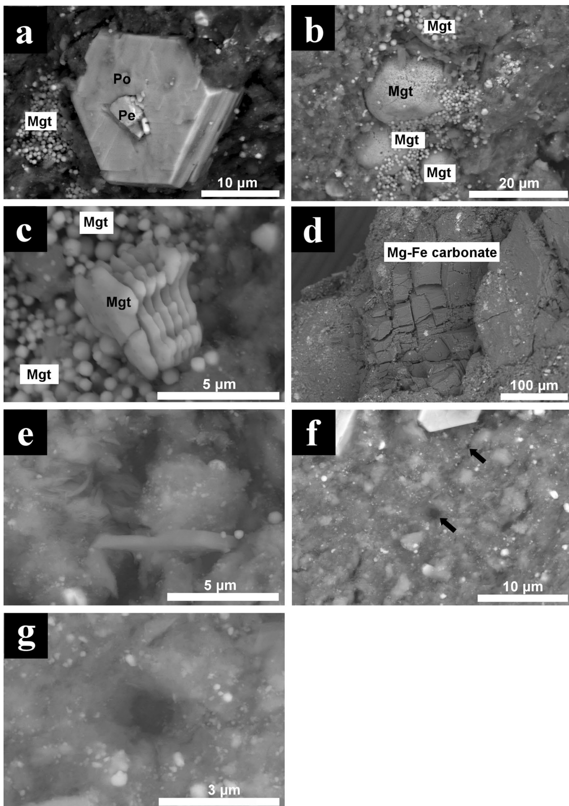
Fig. 8 Back-scattered electron images of major constituent phases in C0041, white group. a Euhedral hexagonal morphology of pyrrhotite showing a smooth texture. b Framboidal magnetite. c Plaquette magnetite. d Large Mg–Fe carbonate. e Coarse-grained phyllosilicate. f Circular structure-enriched region. Larger ones are indicated by arrows. g High-resolution image of a circular structure
