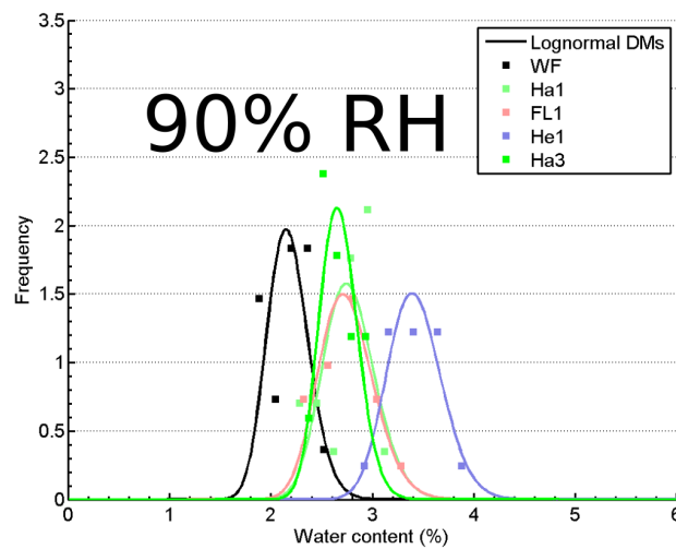
Figure 17: Probability density functions corresponding to the adsorption phase calculated for each RH load and for each formulation - markers are frequencies related the bin-clustering for each mixture (by colour) while continuous curves are least-square adaptation of a lognormal law
