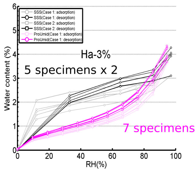
Figure 11: Variability of sorption isotherms for each mix. Case 1 and Case 2 protocols are described in section 2.2.5
