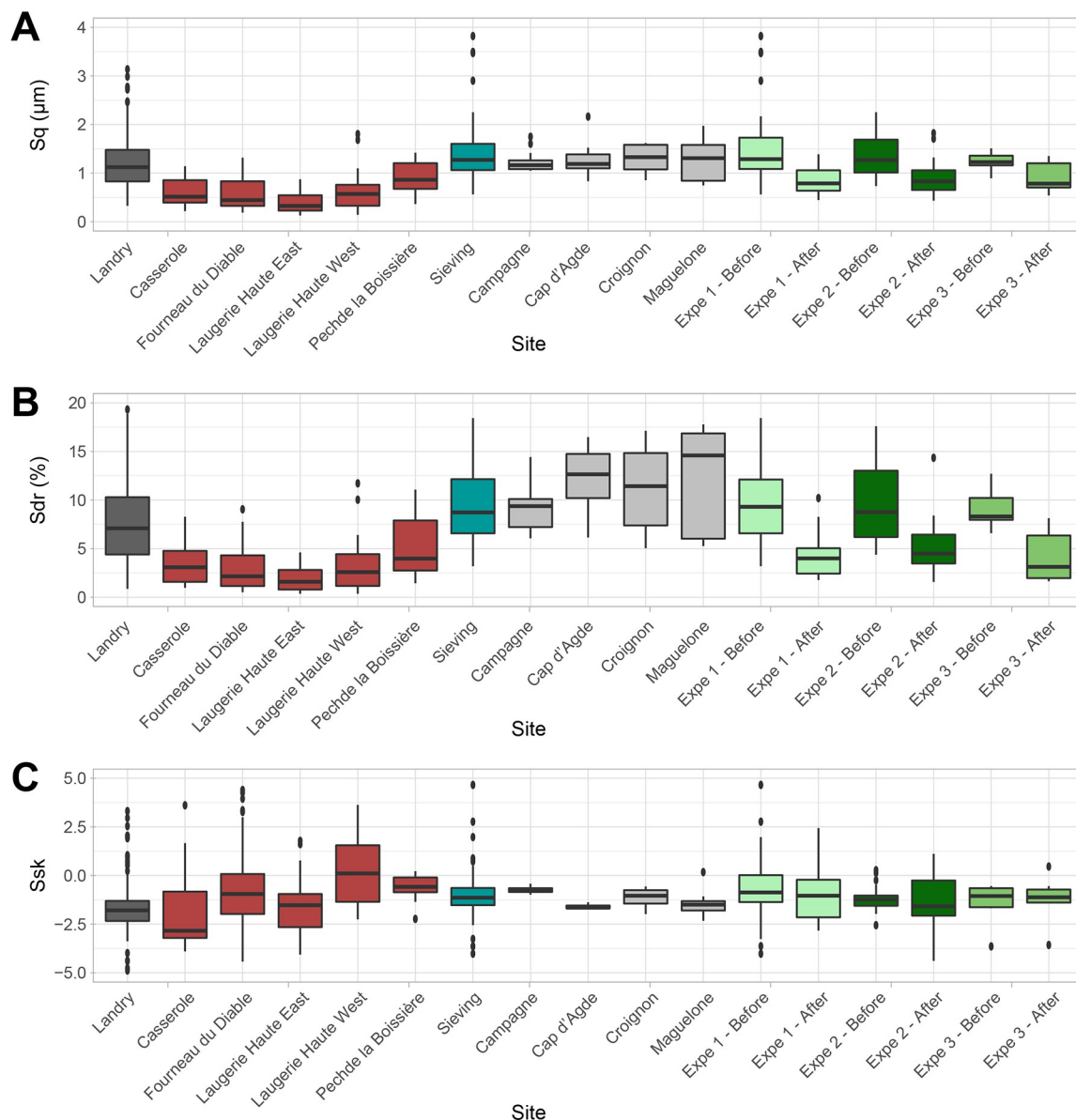
Fig 17. (A) The distribution of Sq (μm) parameter, (B) the distribution of the Sdr (%) parameter and (C) the distribution of Ssk parameter.
