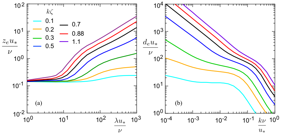
Figure 6: (a) Dimensionless effective hydrodynamic roughness z_e u_* / \nu as a function of \lambda u_* / \nu , computed in a self-consistent way for different values of k\zeta (see legend). (b) Resulting equivalent grain size d_e u_* / \nu as a function of k\nu / u_* for different k\zeta (same colour code as in panel a).
