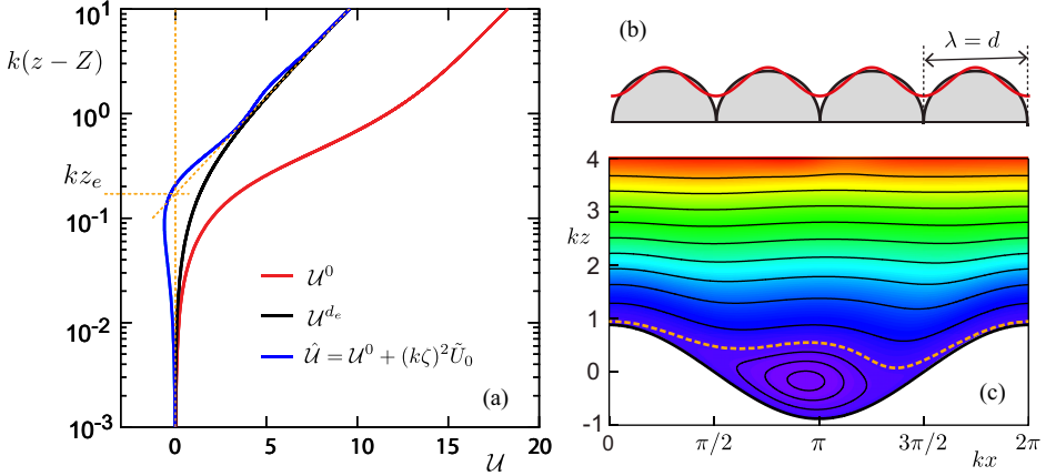
Figure 5: (a) Velocity profiles \mathcal{U}^0 , \hat{\mathcal{U}} and \mathcal{U}^{d_e} introduced in the self-consistent calculation. These two last functions overlap in the upper part of their profiles, i.e. possess the same hydrodynamic roughness z_e (dashed orange lines). Here computation done for k\zeta = 0.88 (see figure 6a) and k\nu/u_* = 0.05 , which converges to d_e u_*/\nu \approx 130 . (b) Sinusoidal approximation of the surface of a periodic array of touching grains, setting \lambda = d . (c) Isocontours of the dimensionless stream function k\Psi/u_* (see Appendix B) above a modulated surface (in white), when k\zeta = 0.88 and k\nu/u_* = 0.05 . The flow is from left to right. Color code: k\Psi/u_* is increasing from blue to red in the background; and the dashed orange curve corresponds to k\Psi/u_* = 0 .
