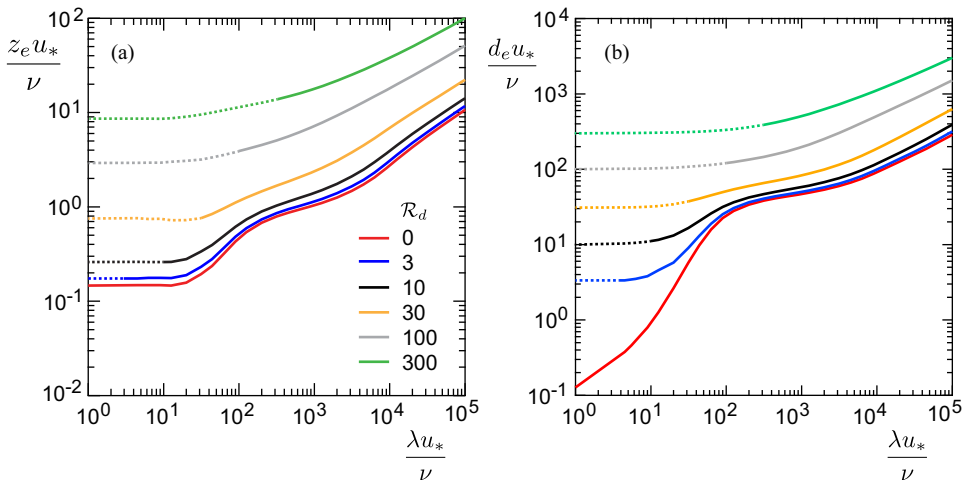
Figure 7: Self-consistent calculation of the effective roughness vs bedform wavelength (a) and the equivalent grain size vs bedform wavelength (b). These are computed for a perturbation of various surface roughness \mathcal{R}_d encoded by different colours (see legend for the colour code in both panels) and with an aspect ratio k\zeta \simeq 0.25 , typically representative of sedimentary dunes. Dashed lines correspond to the moment at which \lambda becomes smaller than d .
