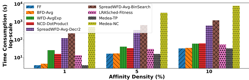
(b) Time consumption - log-scale
