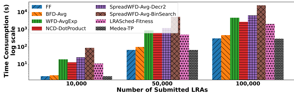
(b) Time consumption - log-scale
