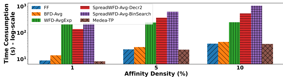
(b) Time consumption - log-scale
