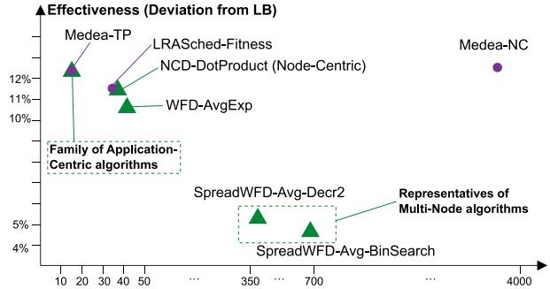
Figure 3: Performance summary of algorithms for instances with 9, 338 LRAs, different affinity densities and without temporal changes
