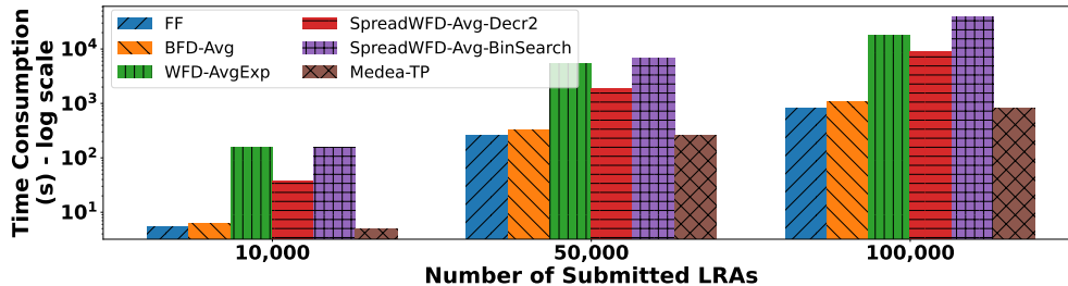
(b) Time consumption - log-scale
