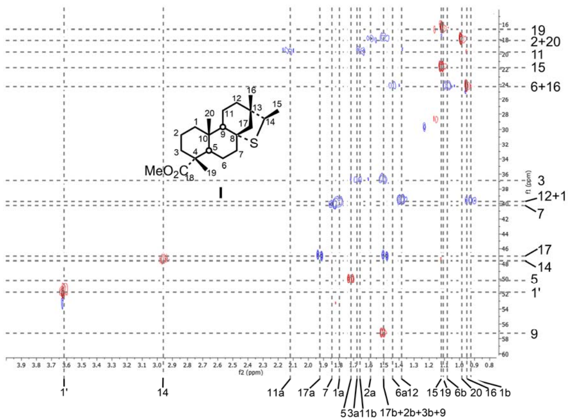
Supplementary figure S6: ^1\text{H} - ^{13}\text{C} one bond ( ^1J ) correlation pattern (HSQC, 500 MHz, \text{CDCl}_3 )
