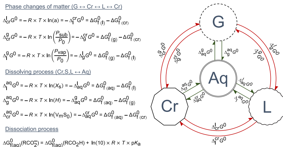
Fig. 1. Thermodynamic cycle resuming the phase-transition (red arrows) along with the dissociation process (green arrows) equations. Formula and related thermodynamic concepts were taken from various articles where they are further discussed [73–79]. At given conditions of temperature, the properties of thermodynamic processes are interrelated, such as, for example: \Delta_{\text{l}}^{\text{g}}G^0 = \Delta_{\text{g}}^{\text{l}}G^0 - \Delta_{\text{Cr}}^{\text{l}}G^0 , \Delta_{\text{Cr}}^{\text{g}}G^0 = \Delta_{\text{g}}^{\text{cr}}G^0 - \Delta_{\text{g}}^{\text{l}}G^0 , and \Delta_{\text{l}}^{\text{aq}}G^0 = \Delta_{\text{g}}^{\text{aq}}G^0 - \Delta_{\text{g}}^{\text{l}}G^0 . Standard Gibbs energies of hydration ( \Delta_{\text{g}}^{\text{aq}}G^0 ), sublimation ( \Delta_{\text{Cr}}^{\text{g}}G^0 ) and dissociation ( \Delta_{\text{l}}^{\text{aq}}G^0 ) expression were applied in this study to calculate a number of Gibbs free energies of formation for various chemicals, by converting them from one phase to another and/or from one form to another. Standard Gibbs free energies formula for other processes were also featured to support further investigations, i.e., \Delta_{\text{aq}}^{\text{l}}G^0 , \Delta_{\text{g}}^{\text{l}}G^0 , \Delta_{\text{l}}^{\text{g}}G^0 , \Delta_{\text{aq}}^{\text{g}}G^0 , \Delta_{\text{Cr}}^{\text{g}}G^0 , \Delta_{\text{Cr}}^{\text{l}}G^0 , \Delta_{\text{g}}^{\text{cr}}G^0 , \Delta_{\text{g}}^{\text{aq}}G^0 , \Delta_{\text{g}}^{\text{l}}G^0 , and \Delta_{\text{l}}^{\text{aq}}G^0 . In these equations, a is the activity of the compound in its solid phase, H represents the Henry's law constant (mol L ^{-1} atm ^{-1} ), m the aqueous solubility (mol L ^{-1} ), P_0 the reference pressure (kPa), P_{\text{sub}} the sublimation pressure (kPa), P_{\text{vap}} the vapor pressure (kPa), pK_a the common logarithm of the dissociation constant, \text{RCO}_2^- the carboxylated anion of an ionisable chemical species, \text{RCO}_2\text{H} the carboxylic acid form of an ionisable species, S_0 the intrinsic solubility of a unionized chemical species in a saturate solution (mol L ^{-1} ), V_m the crystalline molar volume (L mol ^{-1} ), X_s the mole fraction aqueous solubility, and \Delta G_{\text{f}}^0(\text{aq}) the standard Gibbs free energy of formation in aqueous solution. Aq: aqueous, Cr: crystalline solid, G: gaseous, L: liquid.
