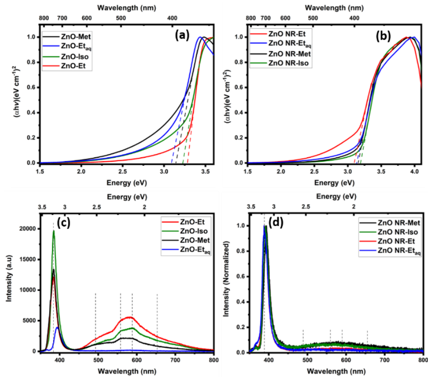
Fig. 7. Tauc plot of samples (a) ZnO-Met, ZnO-Et aq , ZnO-Et and ZnO-Iso and (b) ZnO NR-Met, ZnO NR-Et aq , ZnO NR-Et, and ZnO NR-Iso, (c) PL spectra of samples ZnO-Met, ZnO-Et, ZnO-Et aq and ZnO-Iso and (d) normalized PL spectra of samples ZnO NR-Met, ZnO NR-Et, ZnO NR-Et aq and ZnO NR-Iso.
