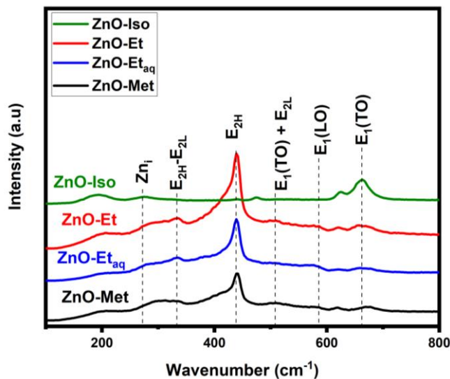
Fig. 6. Raman spectra of samples ZnO-Iso, ZnO-Et, ZnO-Et aq , and ZnO-Met.
