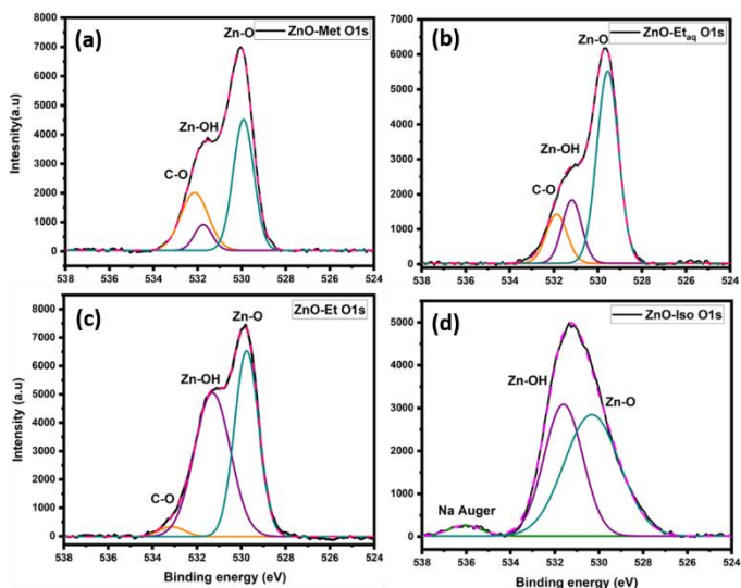
Fig. 5. O1s XPS spectra of samples (a) ZnO-Met, (b) ZnO-Et aq , (c) ZnO-Et and (d) ZnO-Iso.
