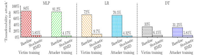
Fig. 4: Evasive malware success rate.
