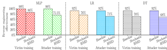
Fig. 3: Reverse-engineering effectiveness.
