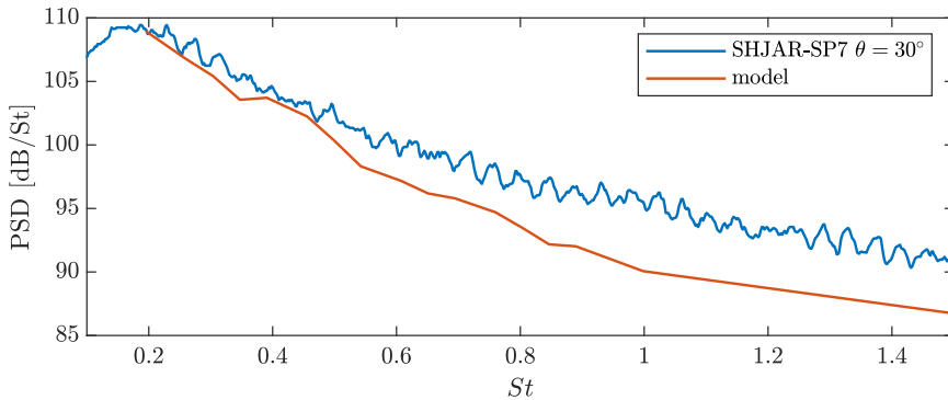
FIGURE 22. PSD of the acoustic pressure at m = 0 predicted by the line-source model (orange) for the NASA-SHJAR-SP7 jet compared against the experimental data for the total acoustic field at \theta = 30^\circ .
