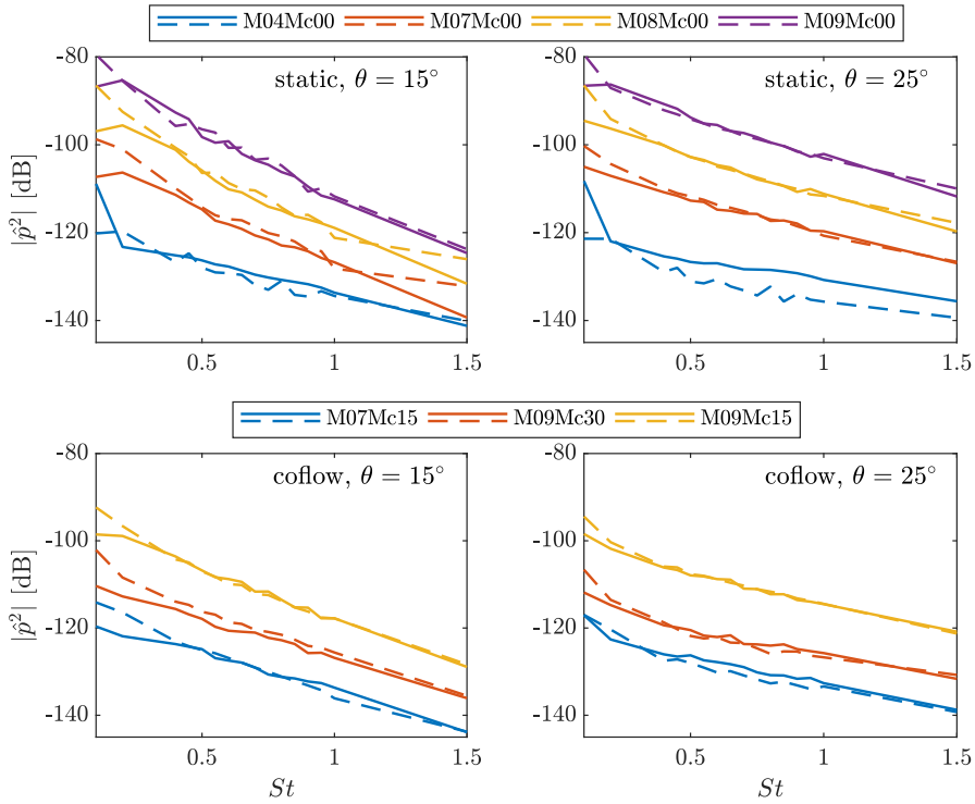
FIGURE 21. PSD of the acoustic pressure obtained from LES (solid) and predicted by the line-source model (dashed) for static jet cases (top) and cases with flight stream (bottom) at two different propagation angles, \theta = 15^\circ (left) and 25^\circ (right).
