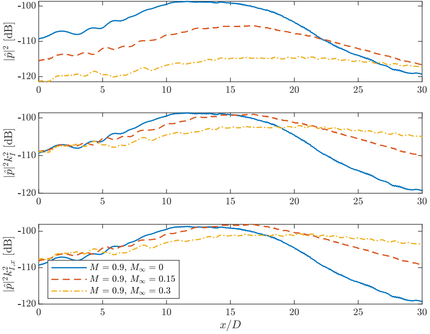
FIGURE 17. PSD of the acoustic pressure for the cases M09Mc00 (solid), M09Mc15 (dashed) and M09Mc30 (dash-dotted) with no scaling (top), k_f^2 scaling (center) and k_{f,x}^2 scaling (bottom) at St = 0.6 .
