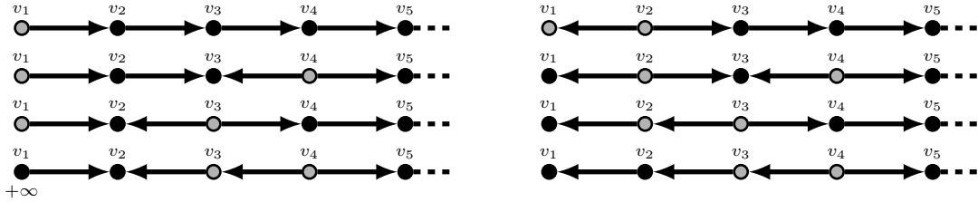
Figure 3: All cases for concluding the proof of Theorem 4.16. For each orientation of P_n , the set of grey vertices is a minimum resolving set. “ +\infty ” below a vertex indicates that this vertex is infinite. Note that, the eight cases when the edge \{v_4, v_5\} is oriented towards v_4 are not depicted. Indeed, in these cases, the grey vertices still distinguish vertices in \{v_1, \dots, v_4\} , while v_5 is distinguished by a resolving set of P' = (v_5, \dots, v_n) .
