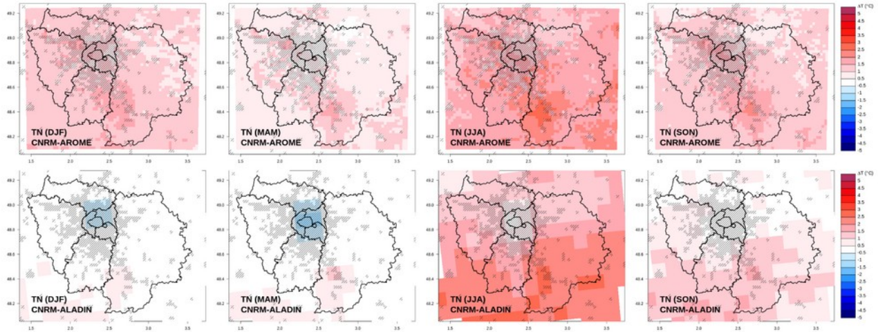
Figure 4: Comparison of seasonal bias maps in TN calculated over the time period 2000-2017 between both CNRM-AROME (top) and CNRM-ALADIN (bottom) simulations and the reference IDF-TNTX database. Hatching represents the extent of Paris urban area (with a cover threshold of 10 % of the CNRM-AROME grid cells, according to the ECOCLIMAP database).
